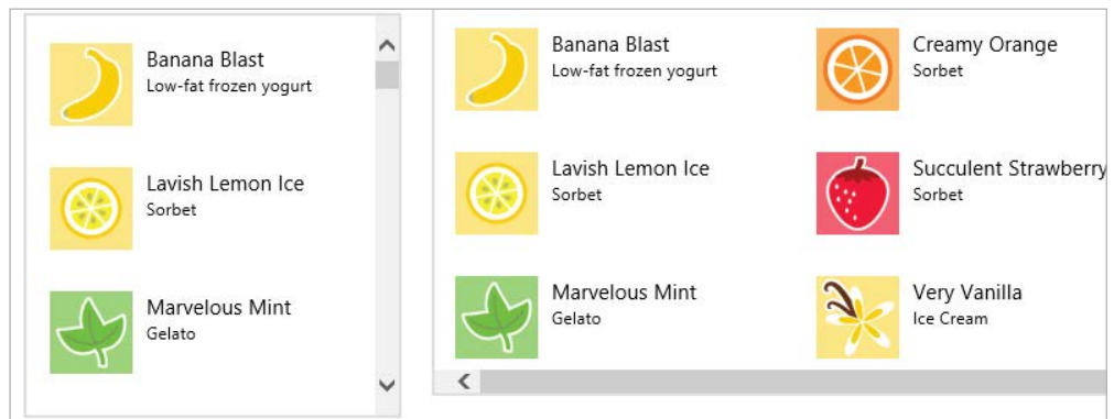
FIGURE 3-4 The List layout on the left and the Grid layout on the right show the same items
