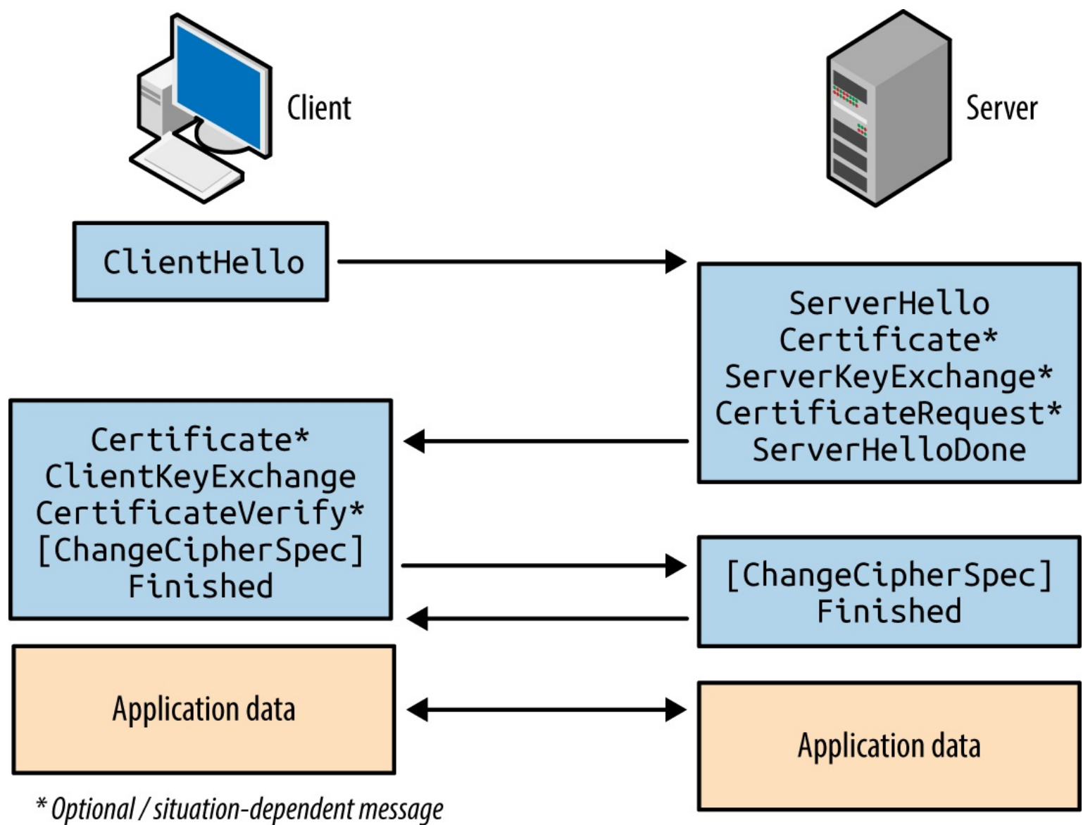
Figure 11-3. TLS handshake message flow
