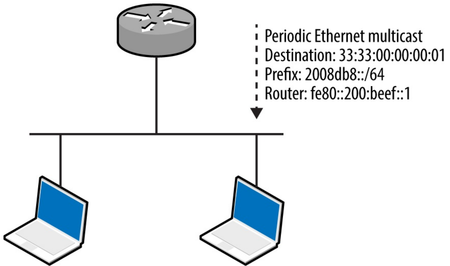
Figure 5-18. IPv6 router advertisement
