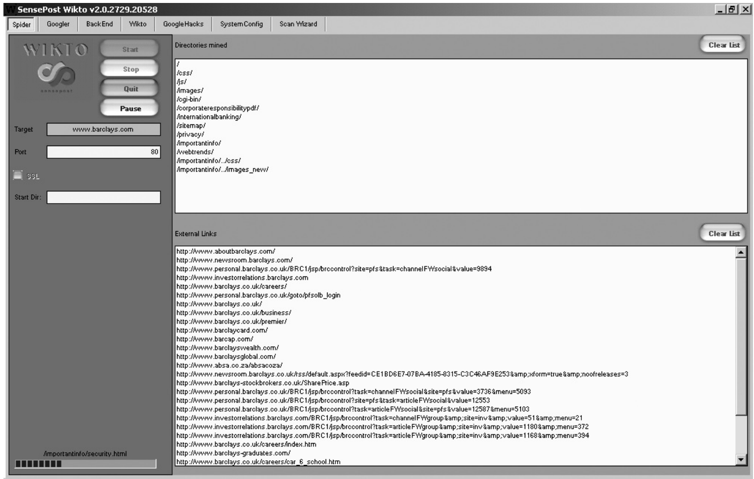
Figure 13-3. Enumerating valid hostnames by using Wikto
