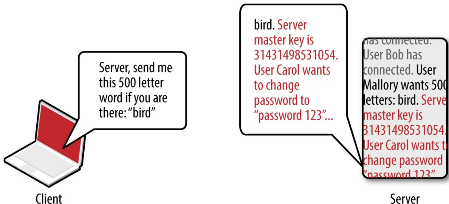
Figure 3-9. A malicious TLS heartbeat request revealing heap content
