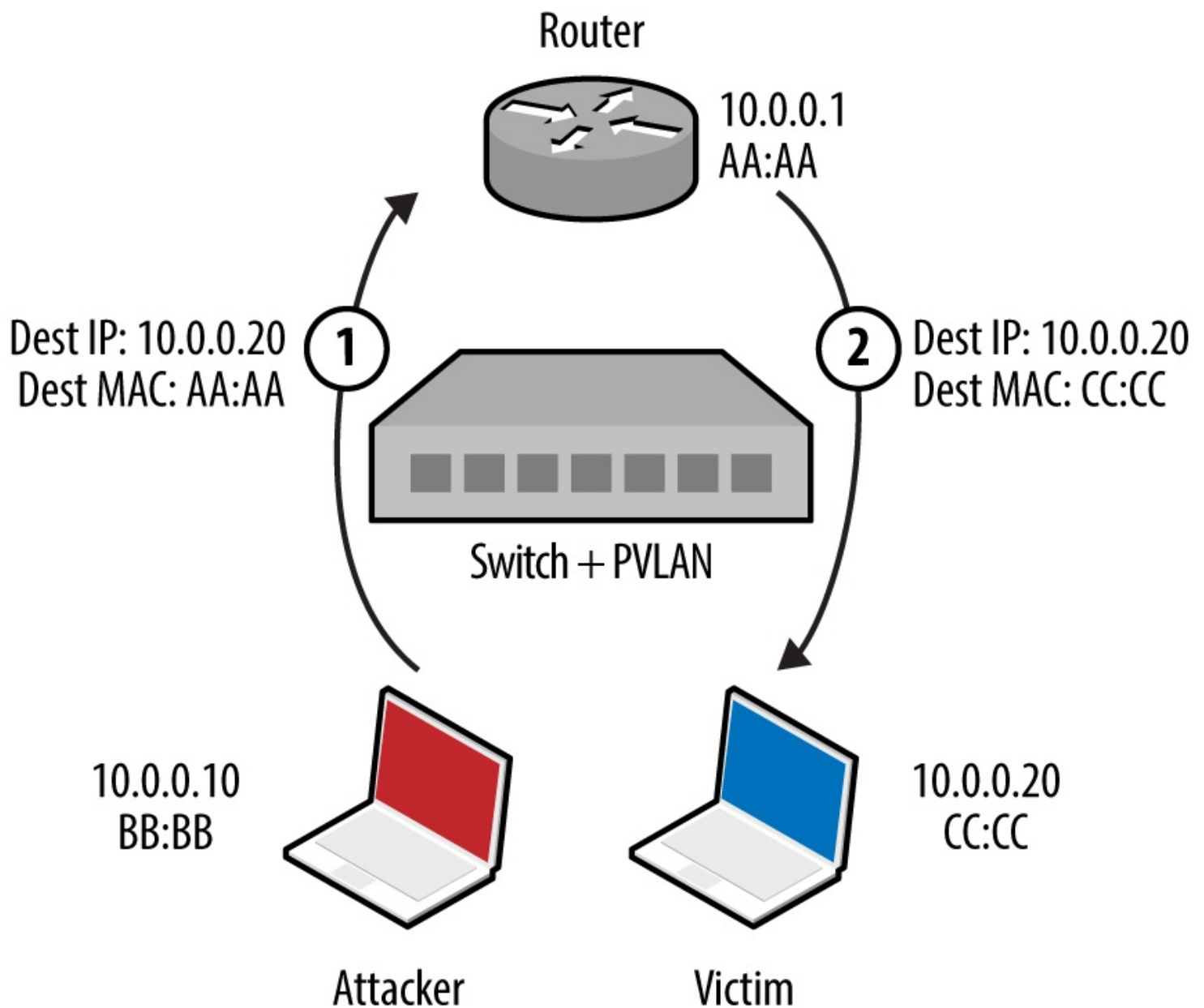
Figure 5-8. A private VLAN attack
