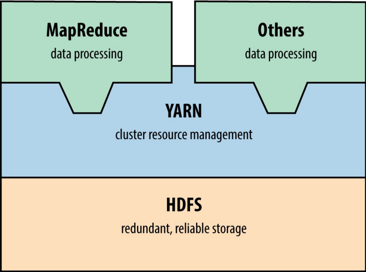
Figure 15-1. Hadoop 2.0 architecture
