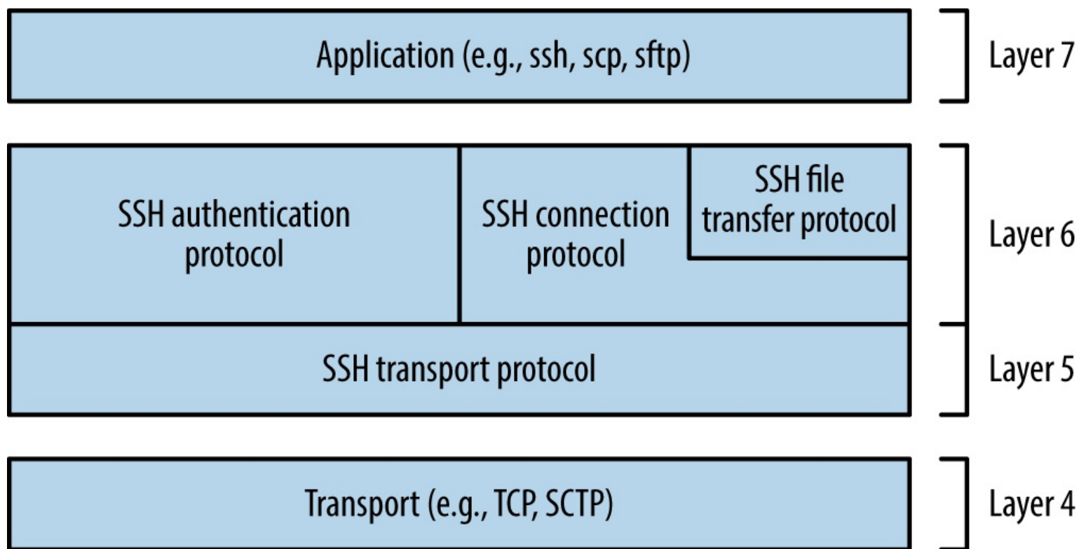
Figure 7-1. SSH 2.0 architecture
