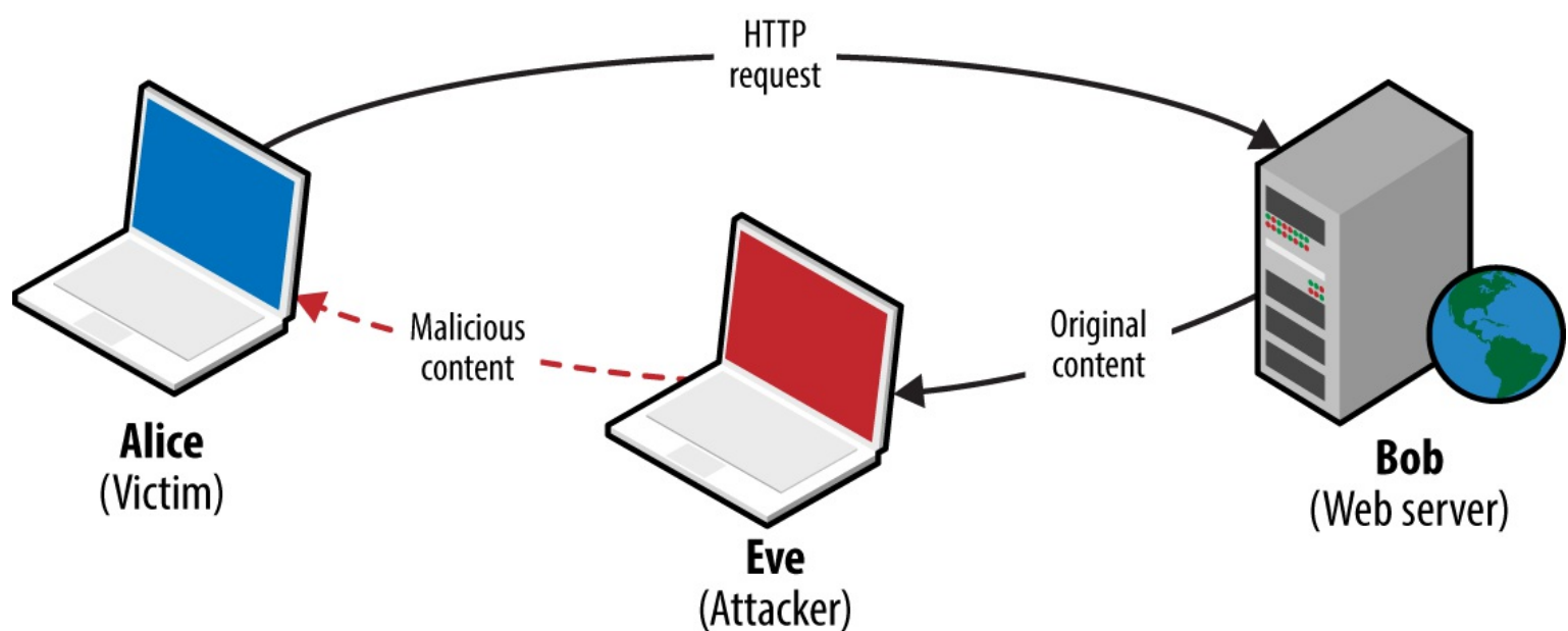
Figure 1-1. Network access used to deliver malicious content
