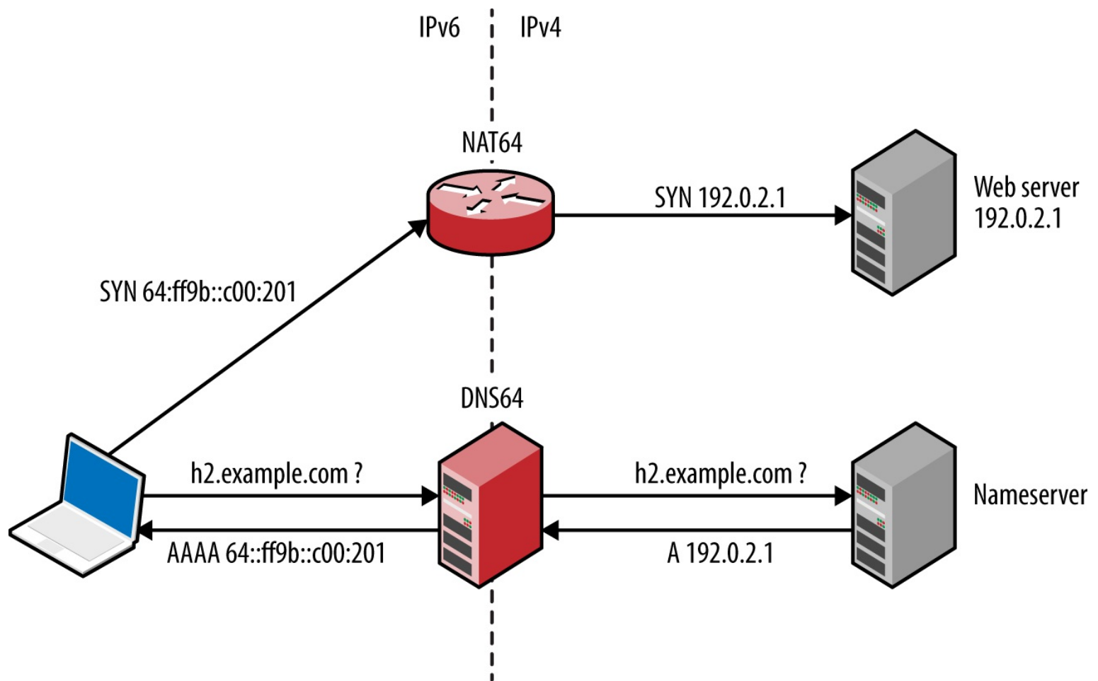
Figure 5-21. Serving IPv6 clients via NAT64 and DNS64
