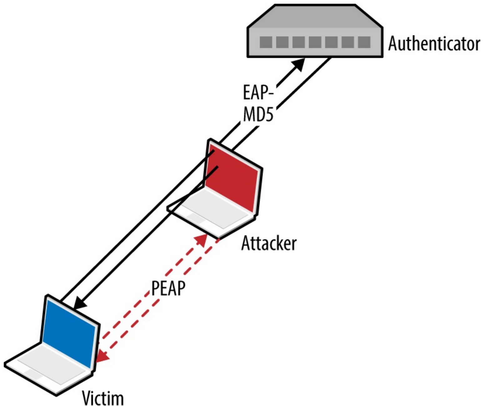
Figure 5-10. Deploying a rogue authenticator
