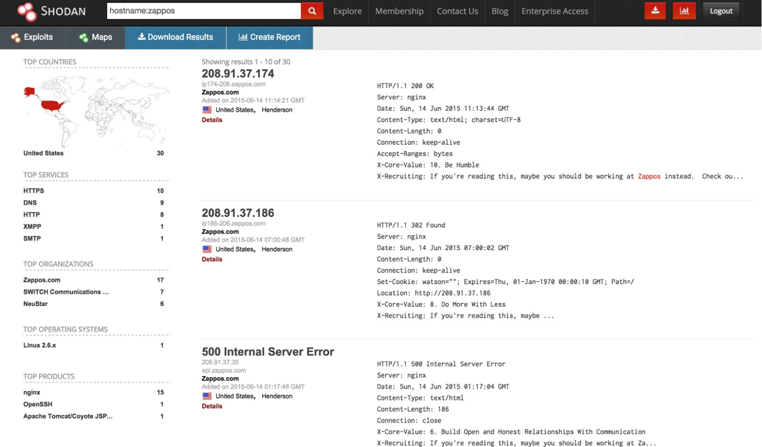
Figure 4-6. Enumerating Internet-exposed services with Shodan
