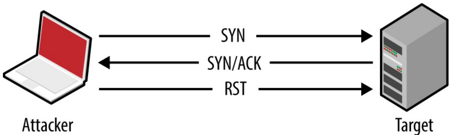
Figure 6-2. Open port behavior
