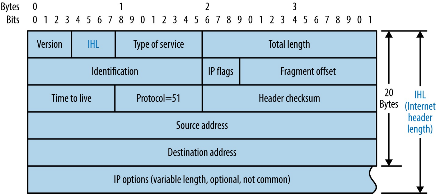
Figure 6-7. IPv4 header format
