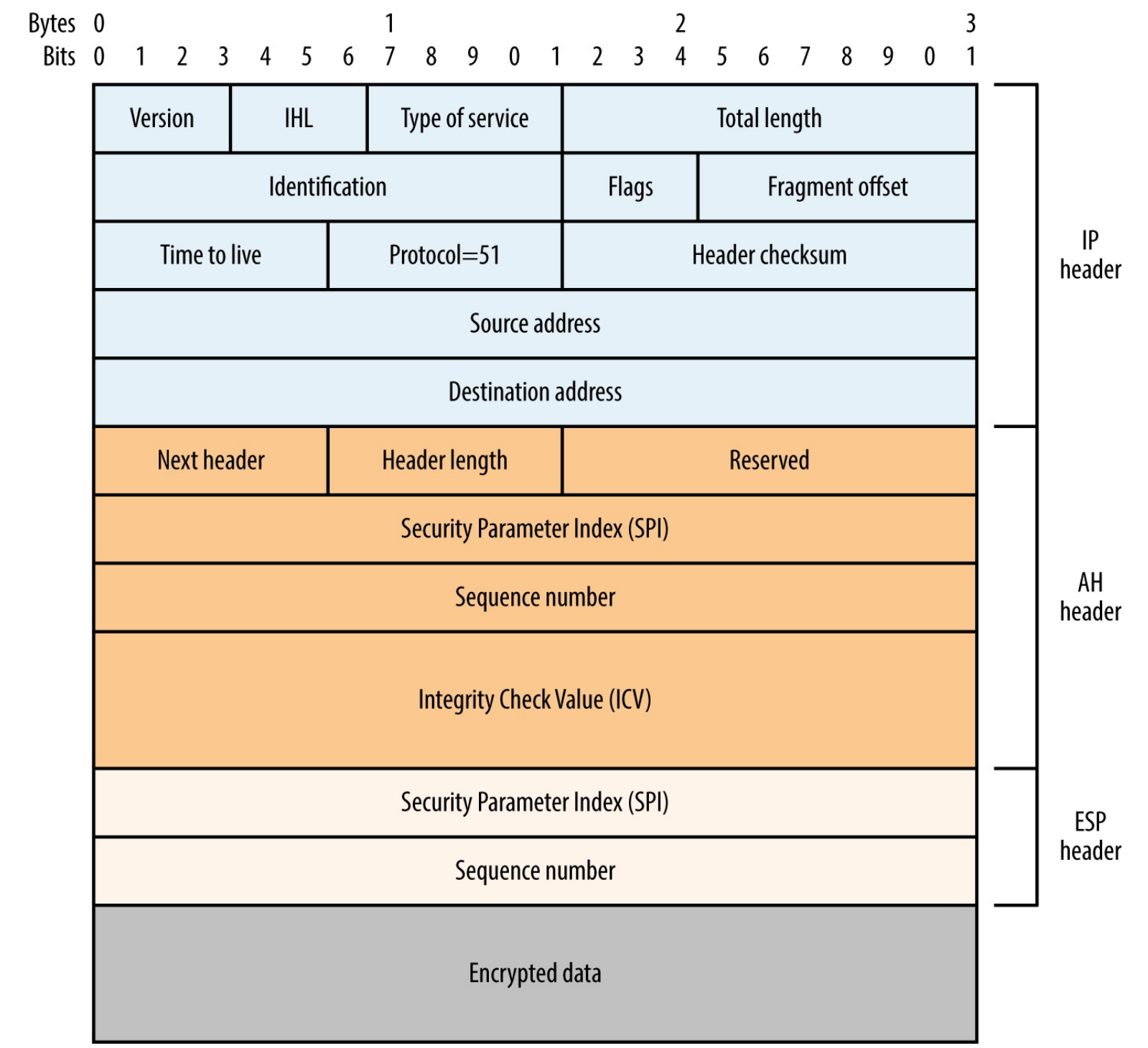
Figure 10-2. IPsec datagram format (tunnel mode)
