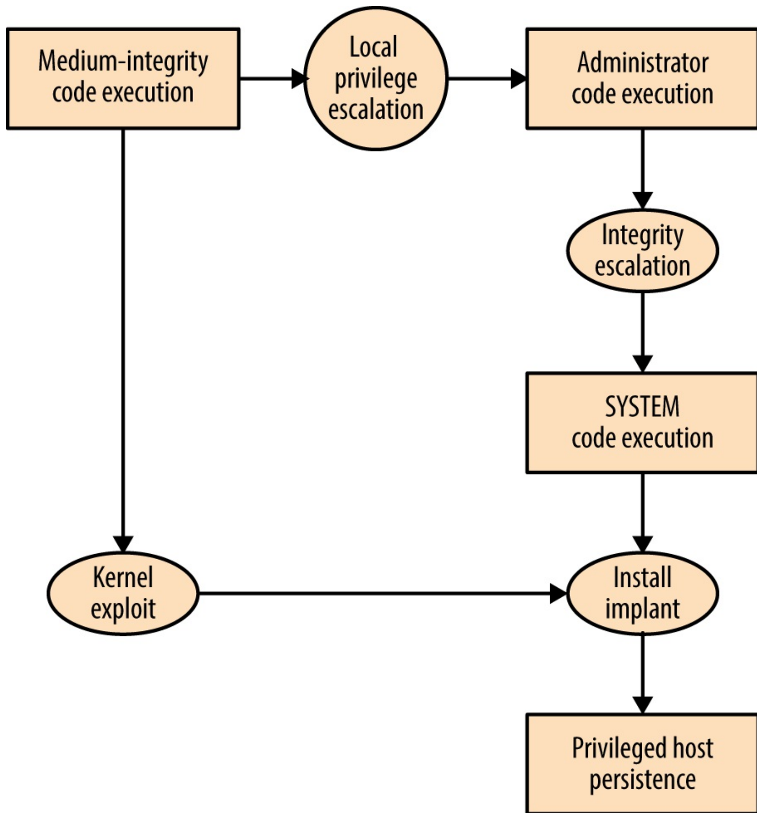
Figure 3-5. Local privilege escalation attack graph
