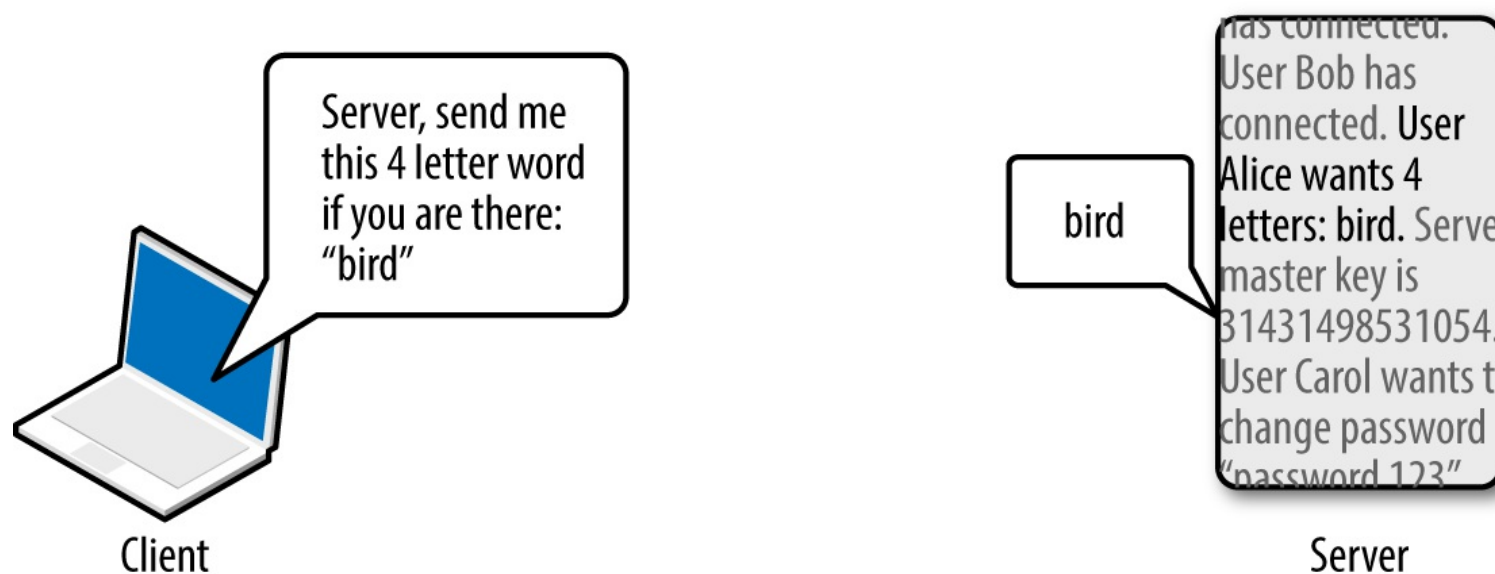
Figure 3-8. A server fulfilling a TLS heartbeat request
