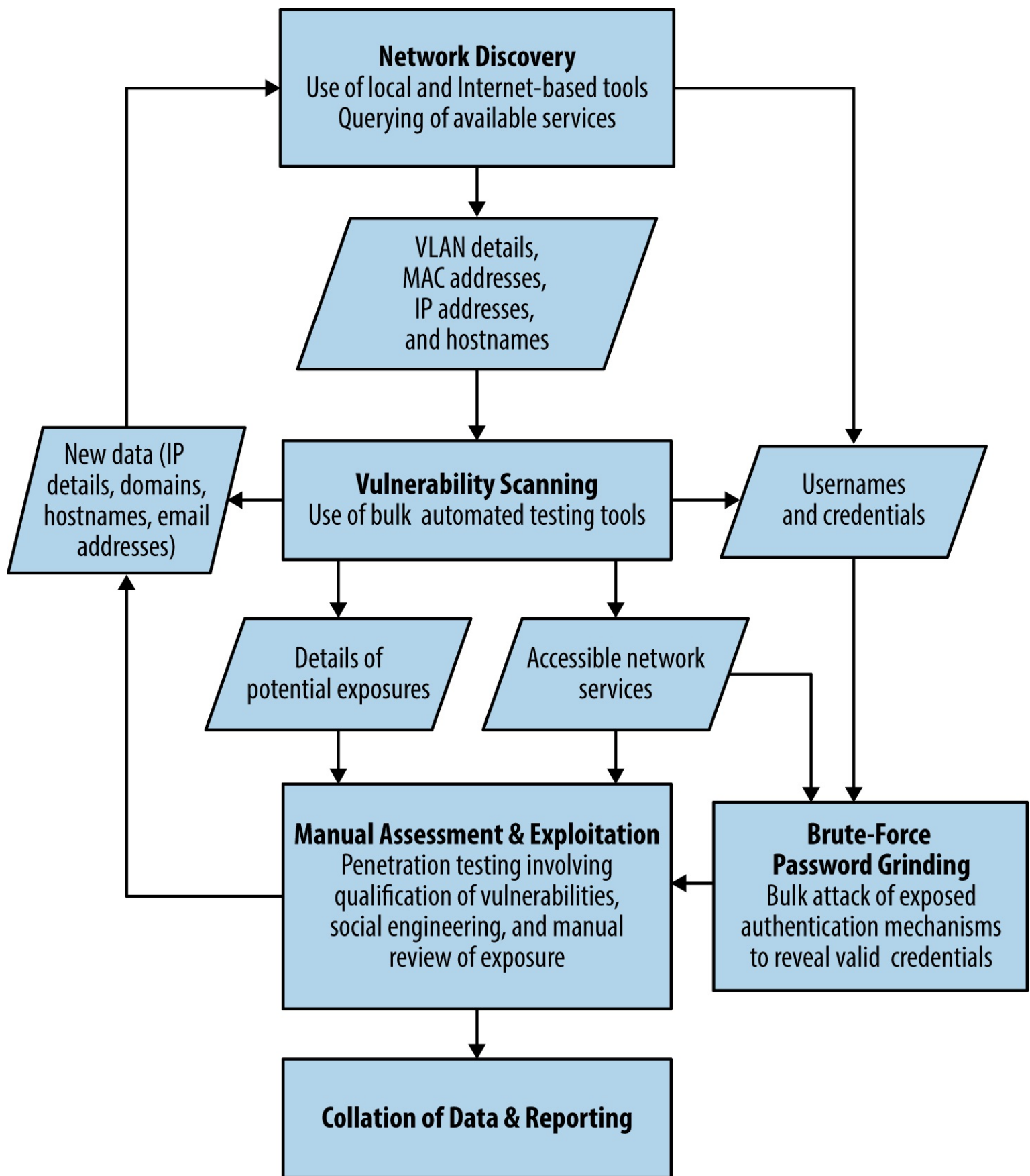
Figure 2-3. An iterative approach to discovery and testing
