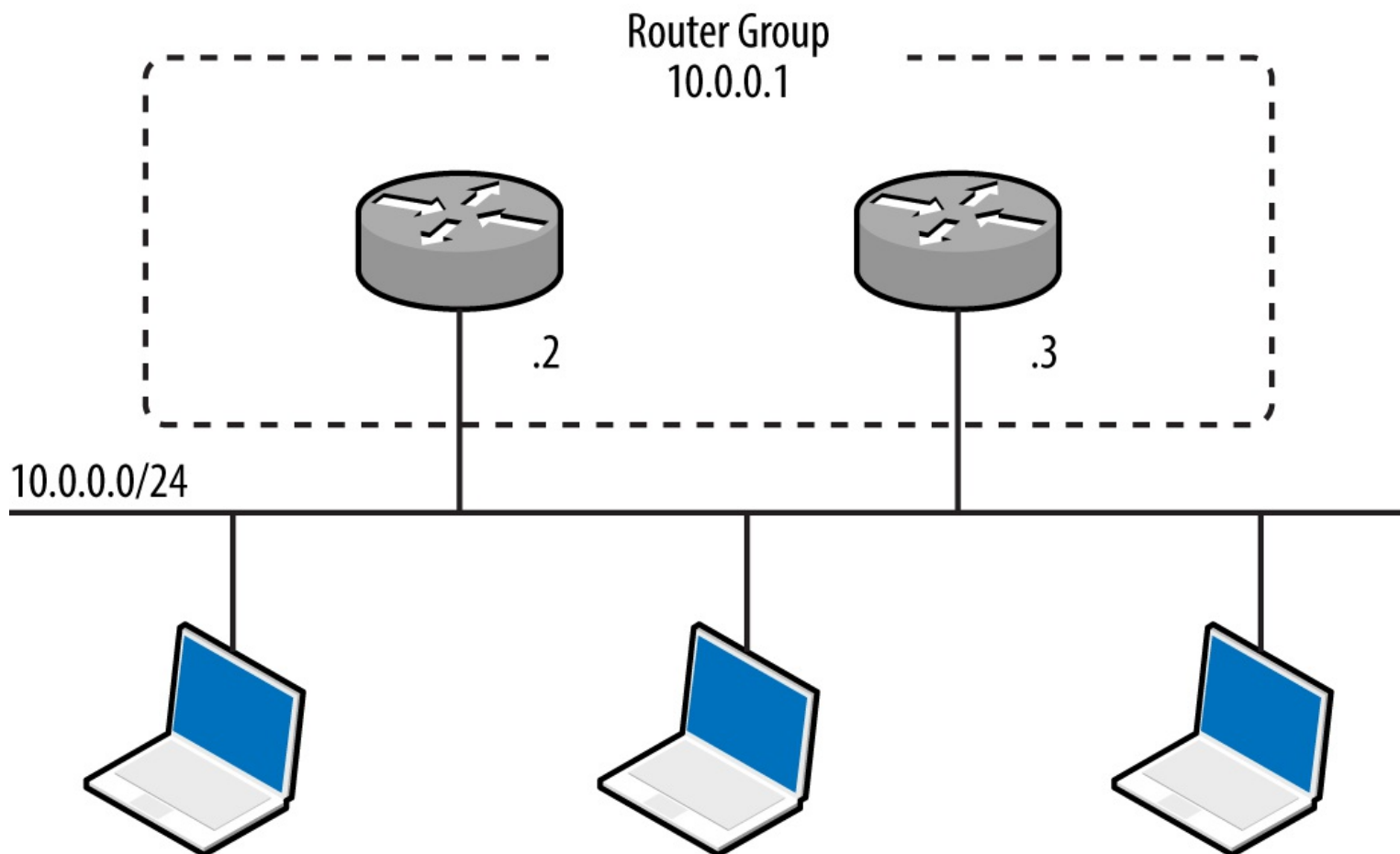
Figure 5-15. A redundant router group
