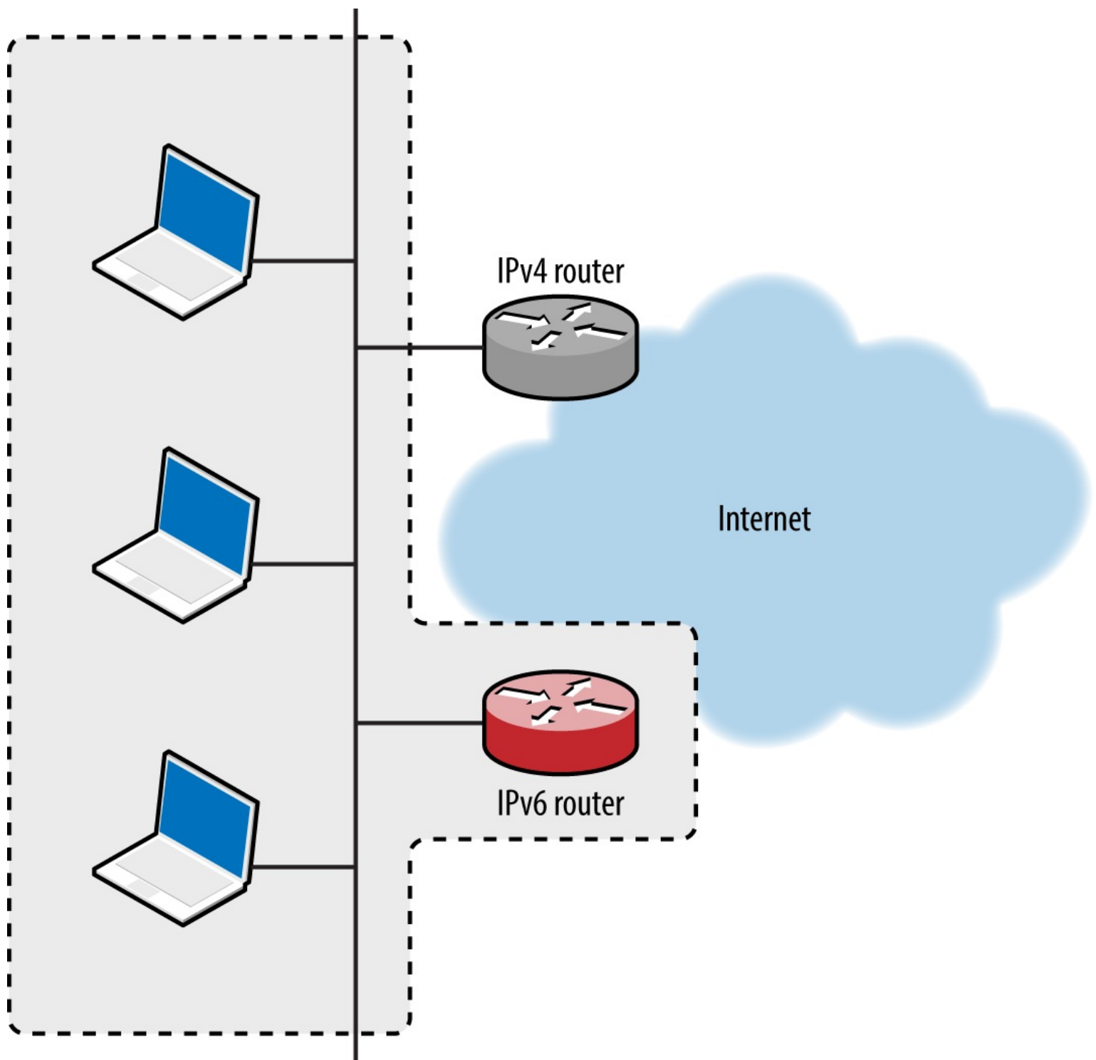
Figure 5-20. Implementing a malicious IPv6 overlay network
