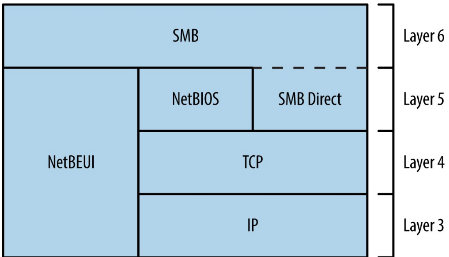
Figure 8-2. SMB is available through different services
