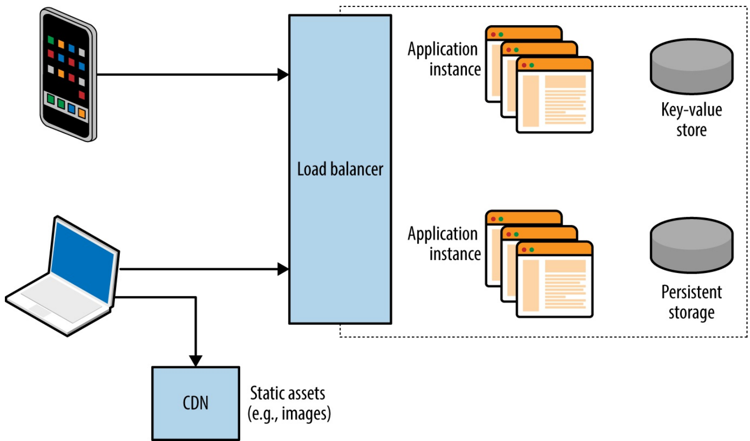
Figure 12-2. A complex web application
