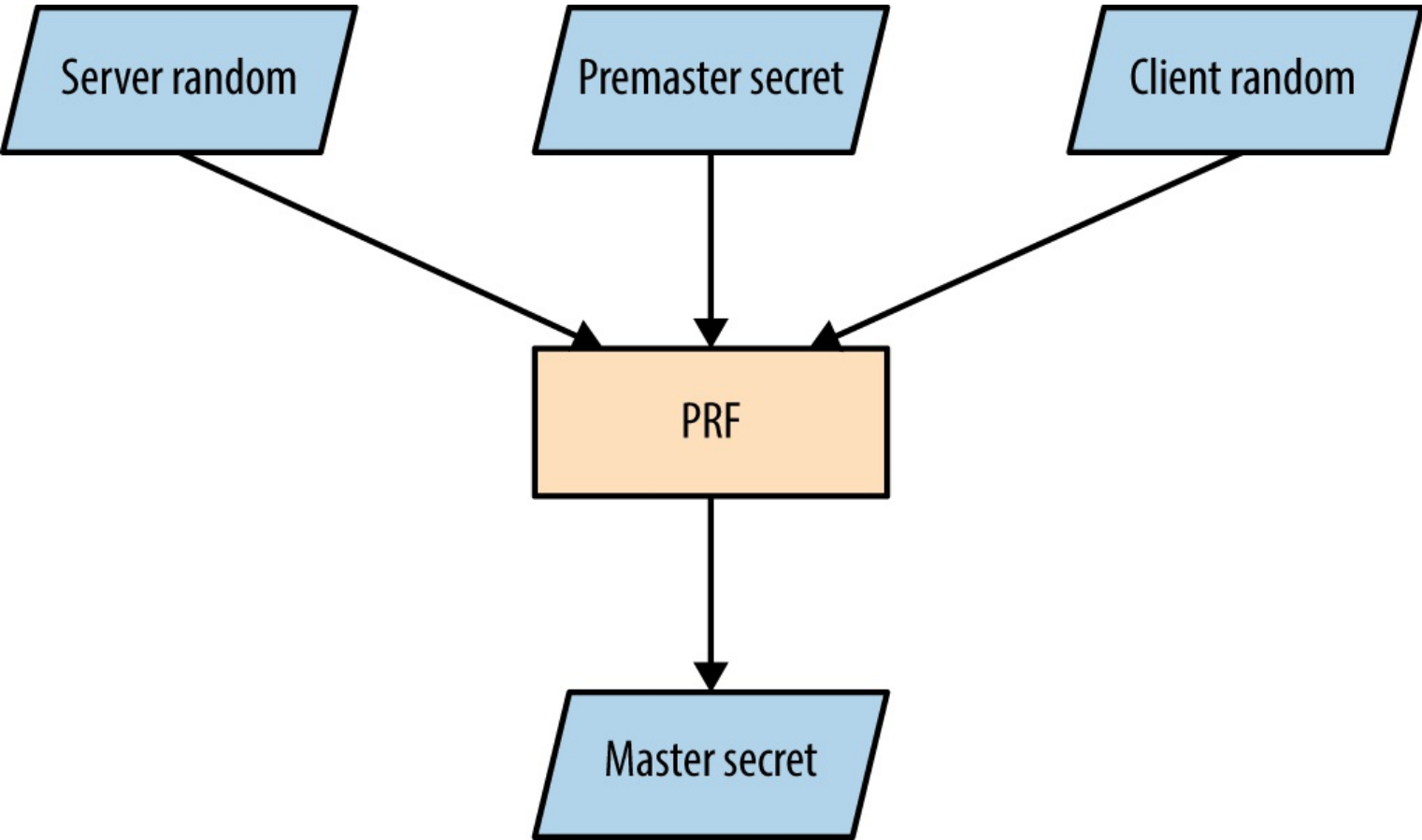
Figure 11-4. Master secret generation
