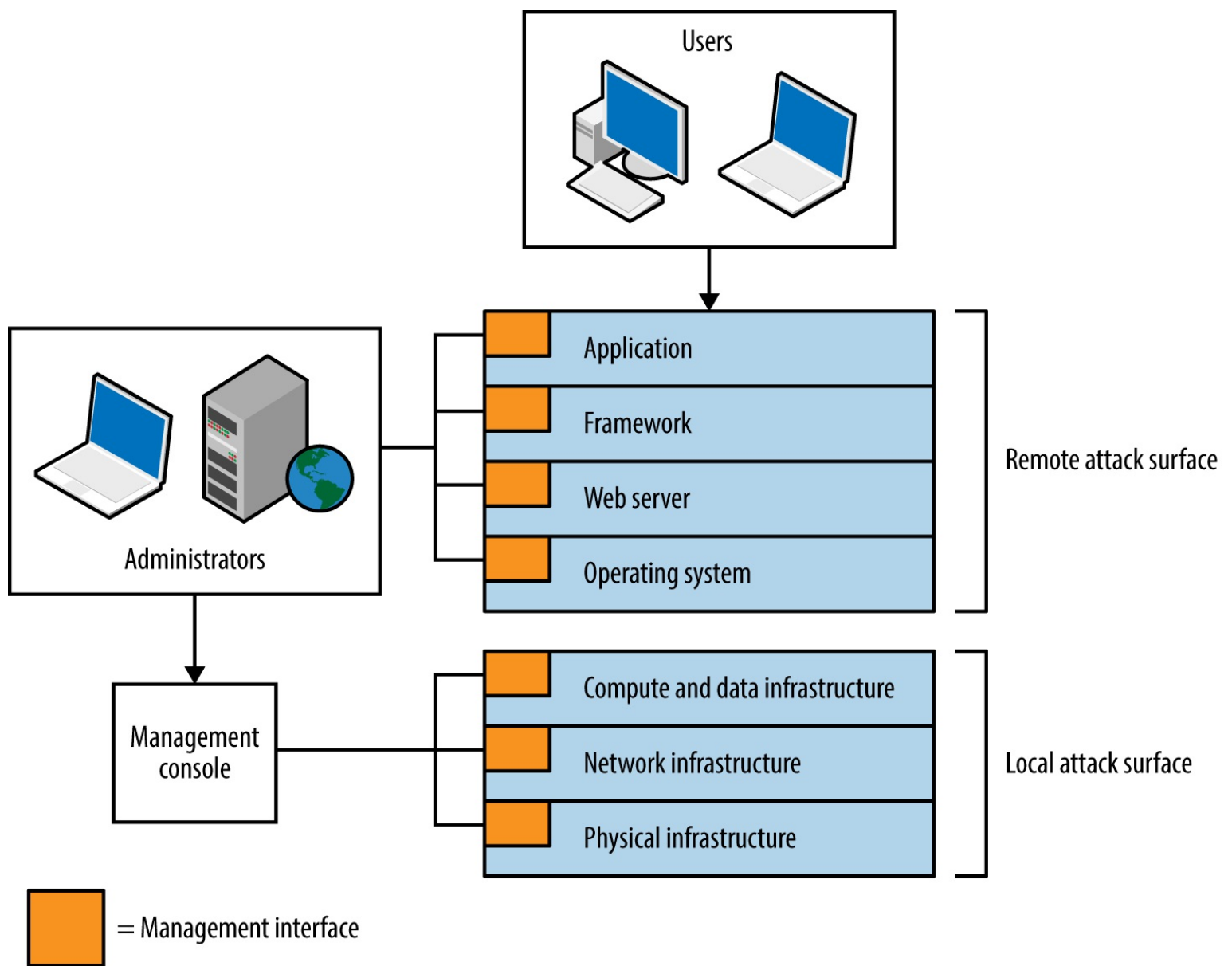
Figure 3-2. Attack surface of a cloud application
