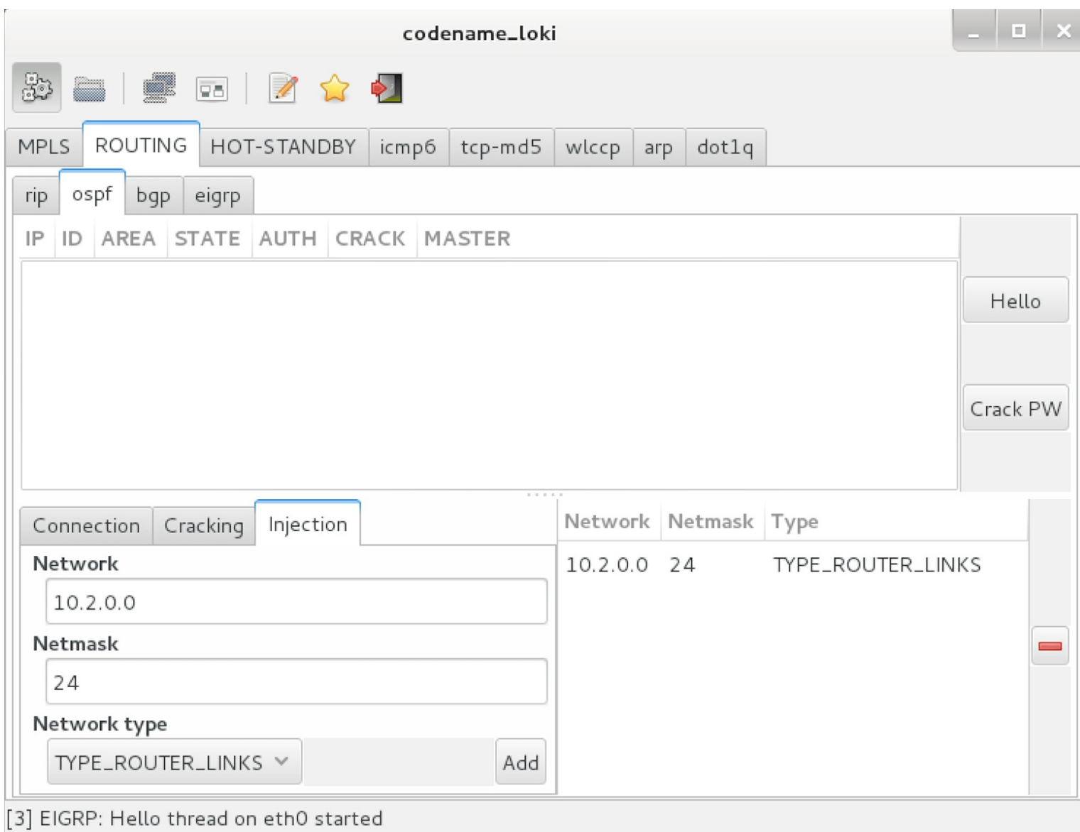
Figure 5-17. Advertising a new OSPF route using Loki
