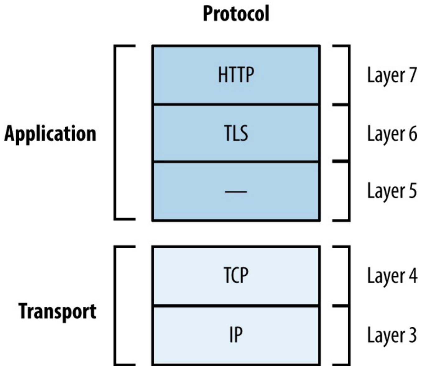
Figure 11-1. TLS belongs to Layer 6
