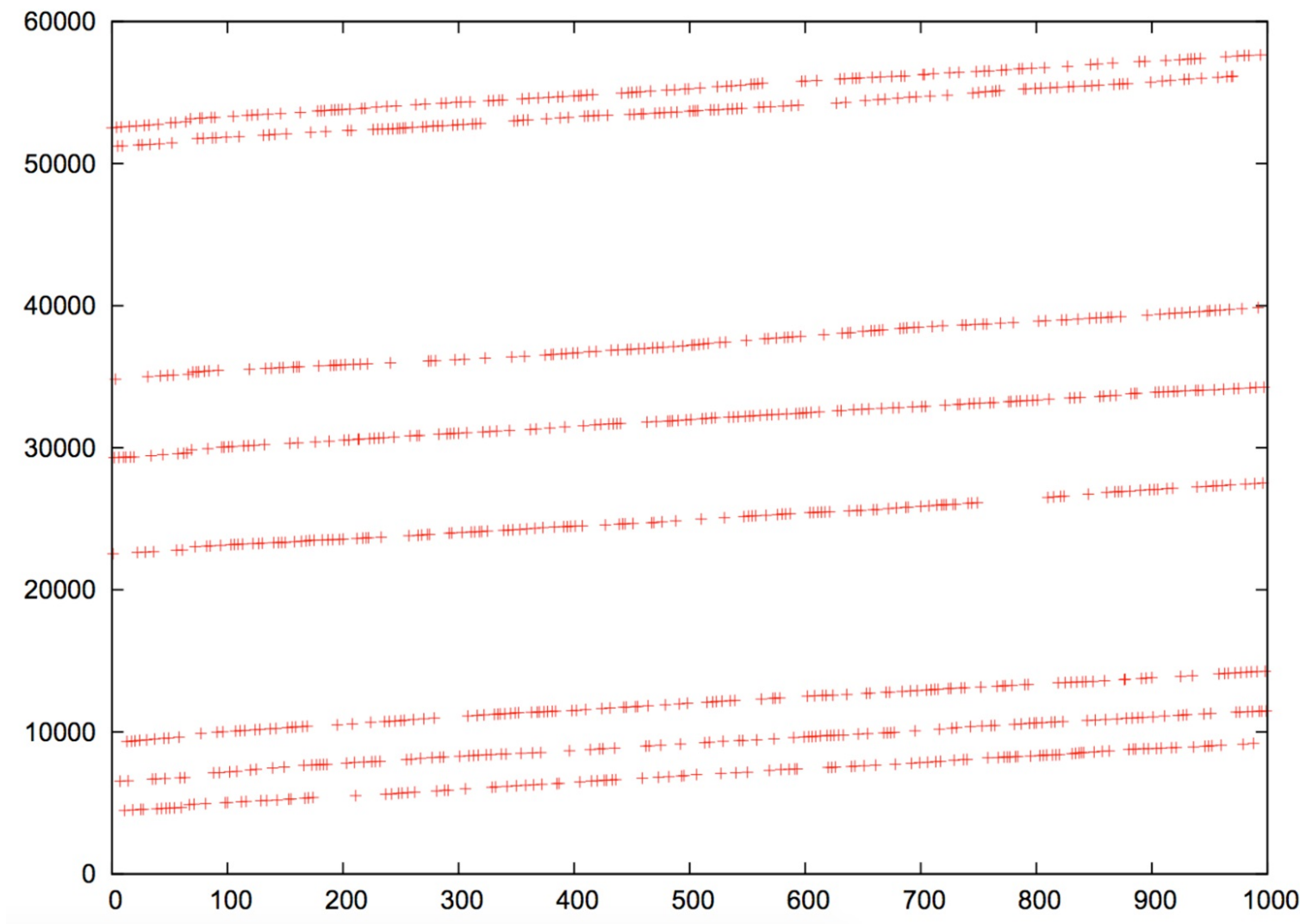
Figure 6-9. IP ID value plot for www.yahoo.fr
