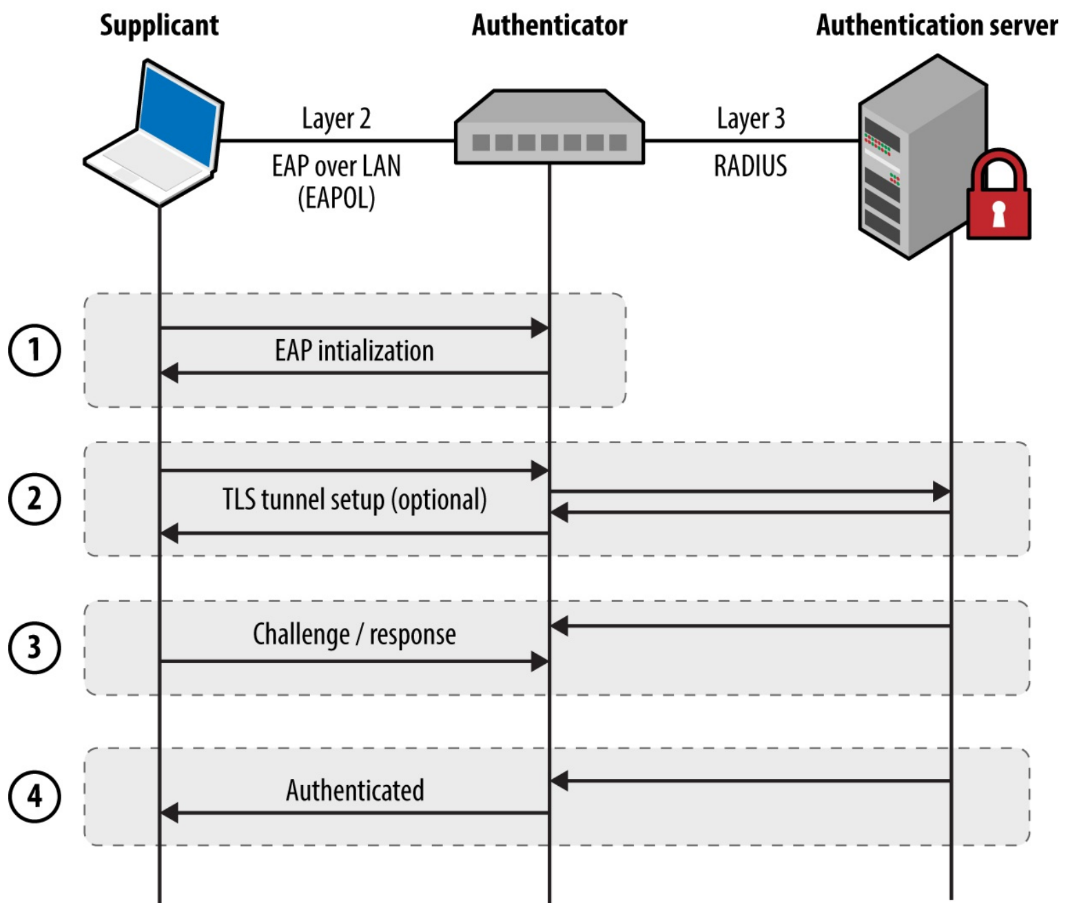
Figure 5-9. 802.1X authentication
