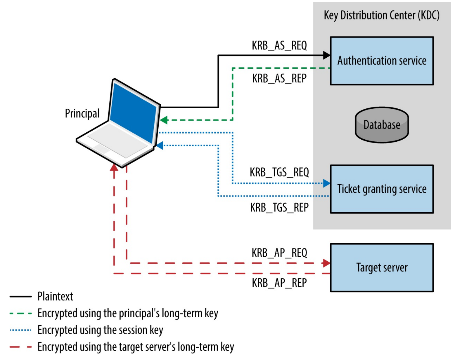
Figure 7-5. Kerberos KDC authentication and ticketing
