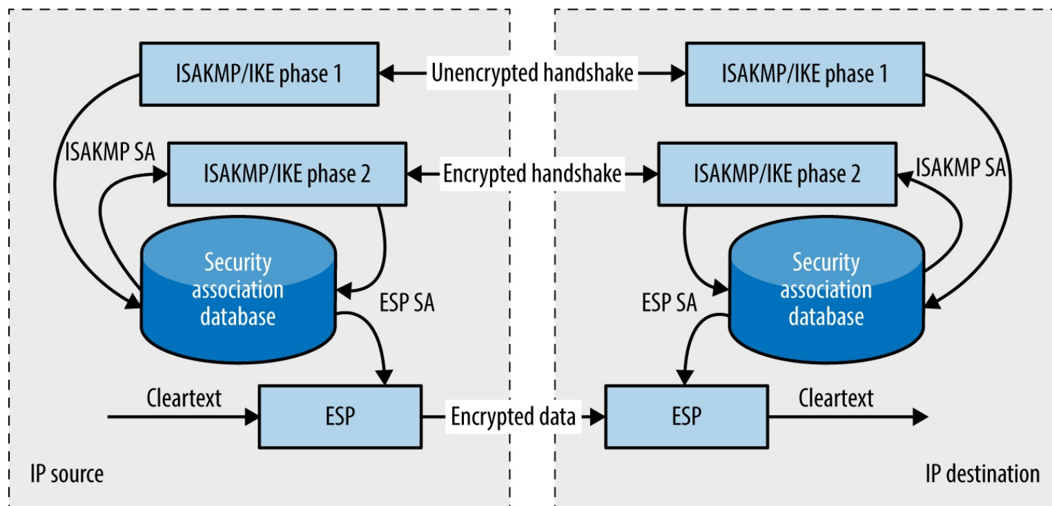
Figure 10-1. Setup and use of an IPsec tunnel with IKE
