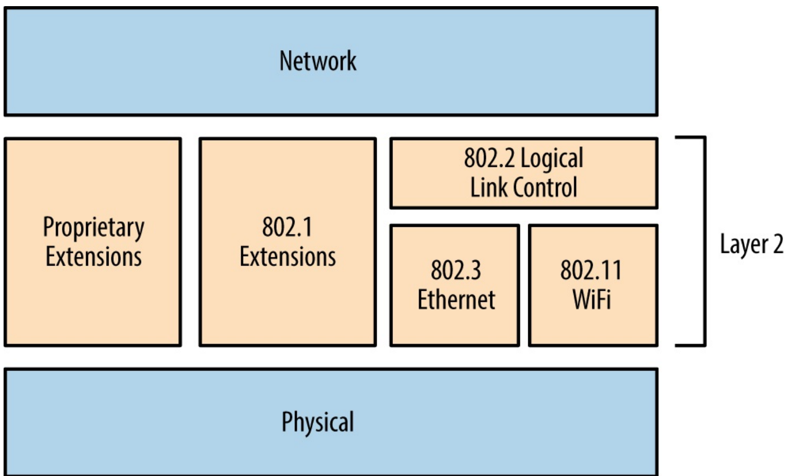
Figure 5-1. The physical, data link, and network layers
