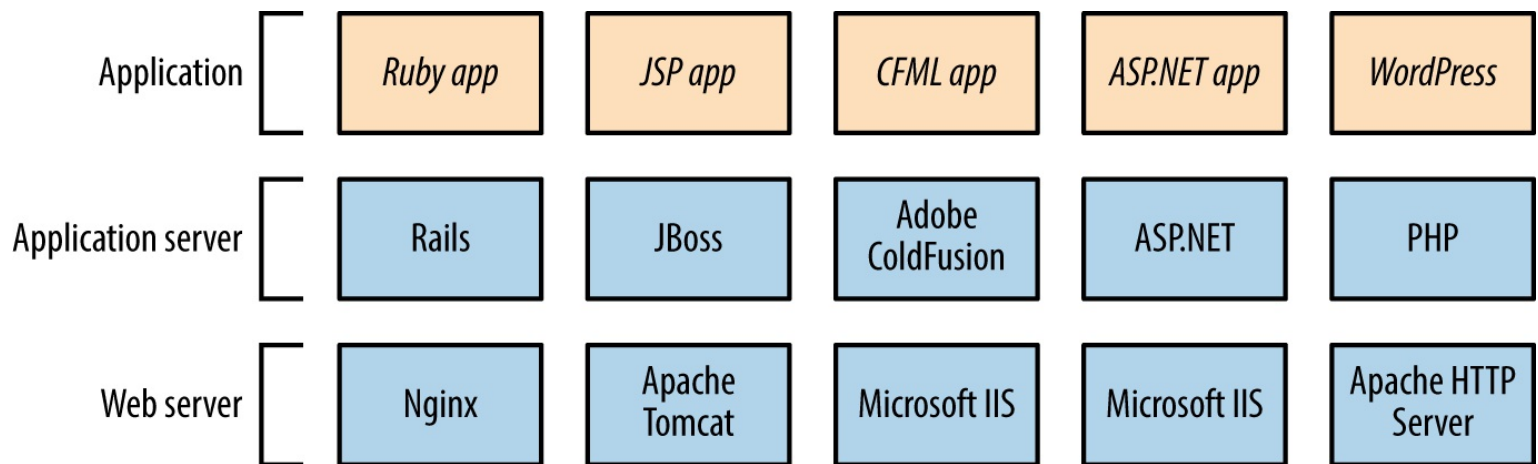
Figure 14-1. Common application framework configurations
