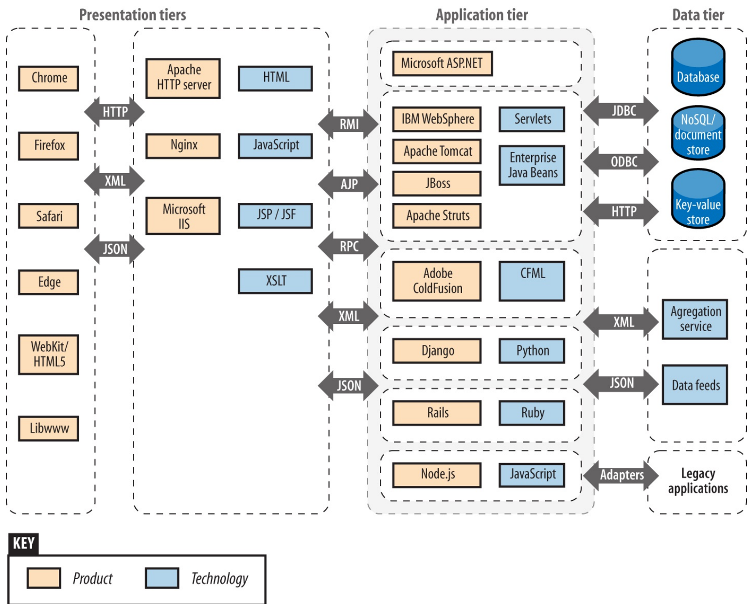
Figure 12-3. Web application technologies and protocols
