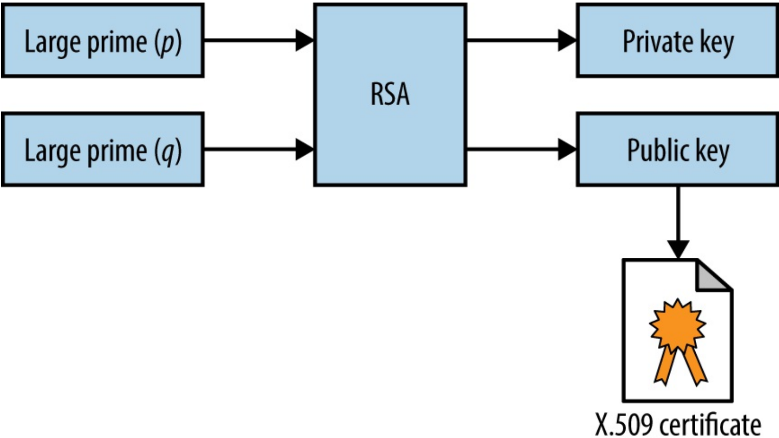
Figure 11-7. X.509 RSA key generation
