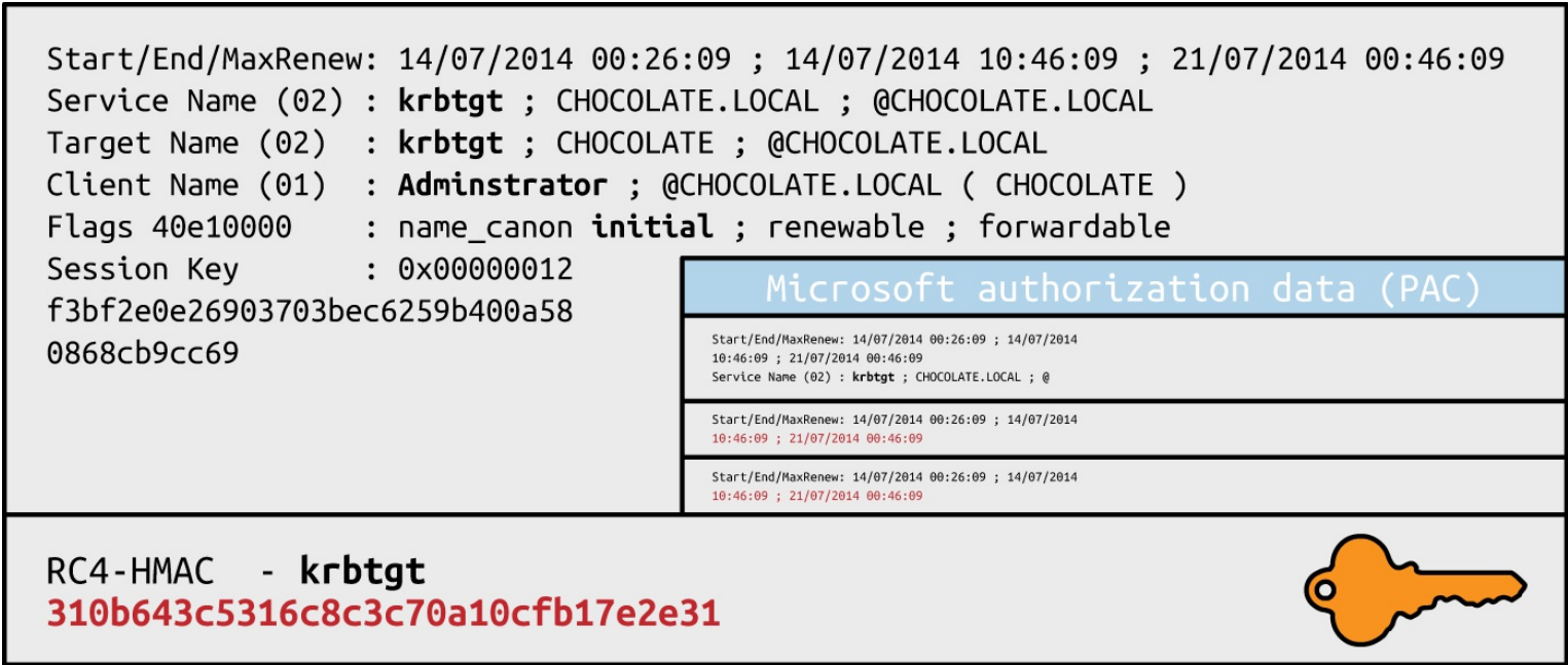
Figure 7-6. Microsoft Kerberos ticket format
