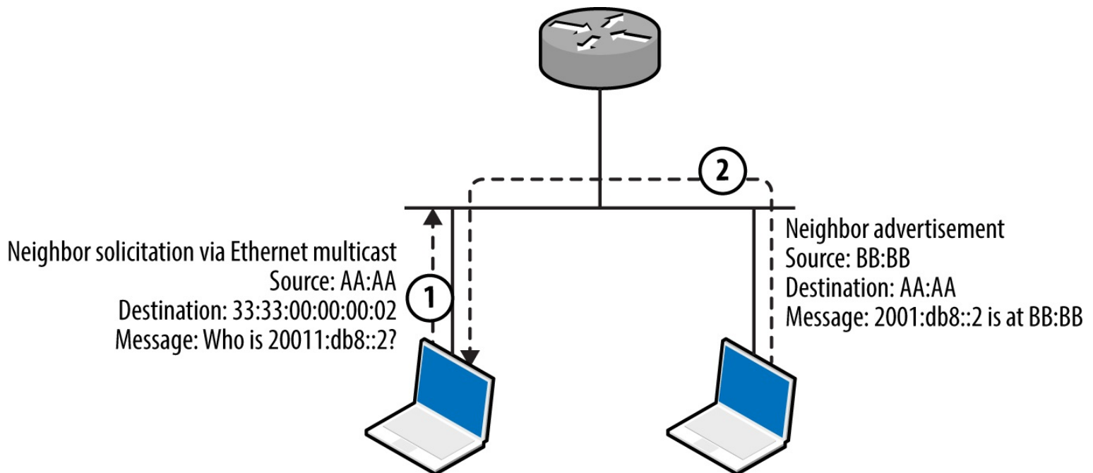
Figure 5-19. IPv6 neighbor solicitation and advertisement
