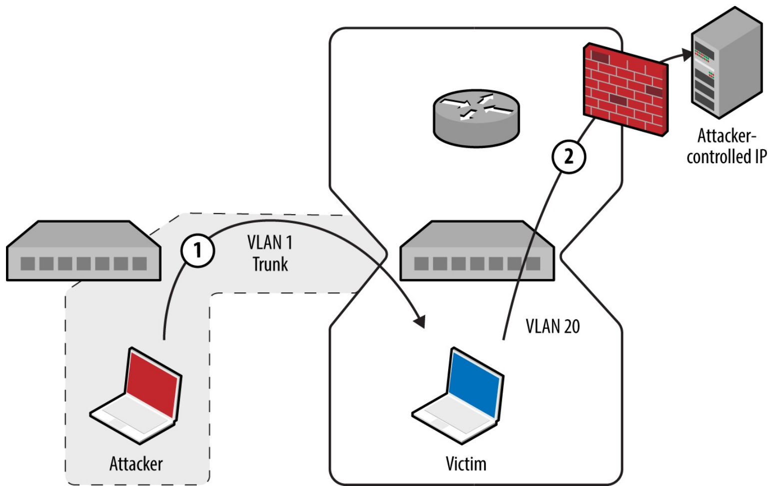
Figure 5-7. Bypassing security controls by double-tagging
