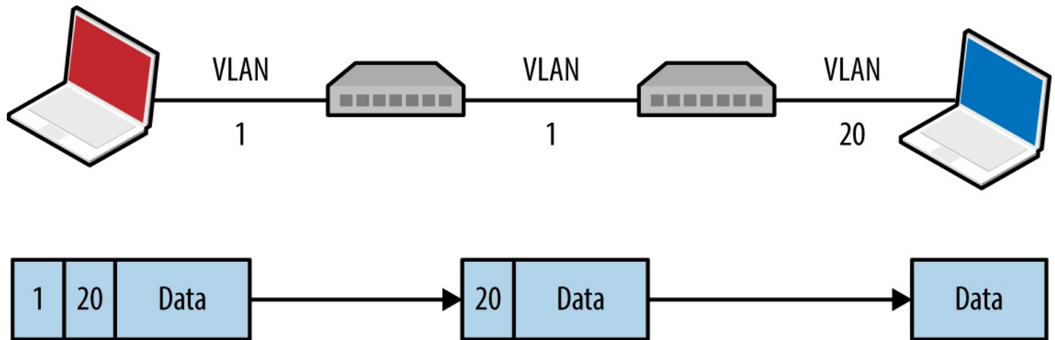
Figure 5-6. Double-tagging VLAN frames
