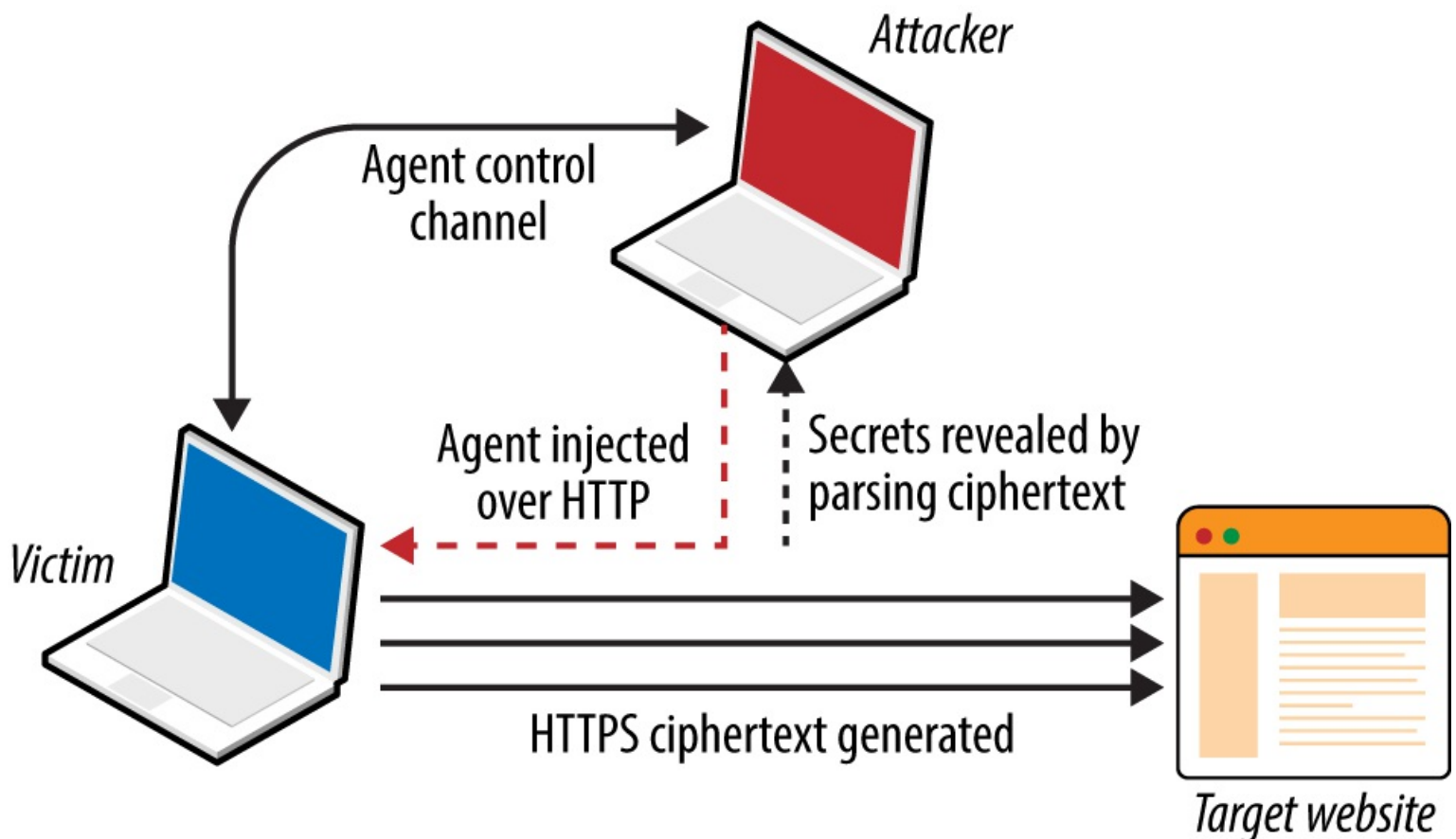
Figure 11-9. Exploiting TLS flaws with network access
