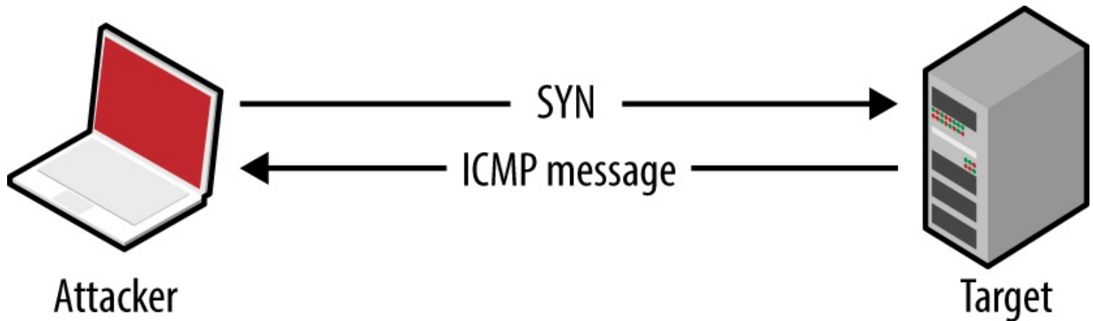
Figure 6-5. Filtered port behavior (ICMP response)
