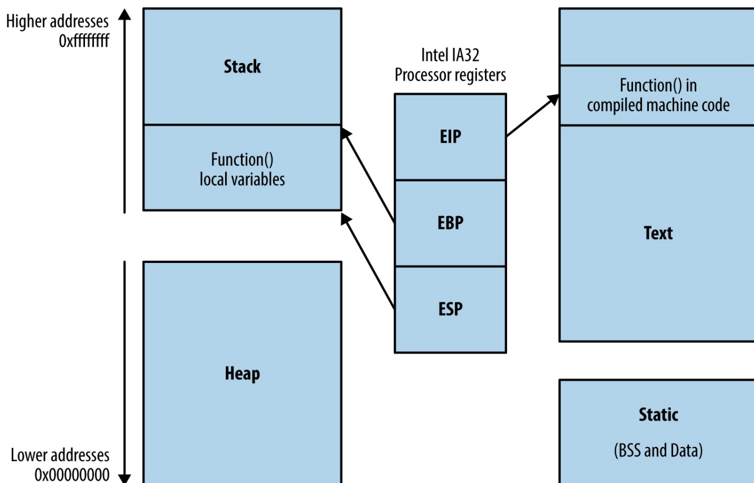
Figure 3-7. Intel processor registers and runtime memory layout
