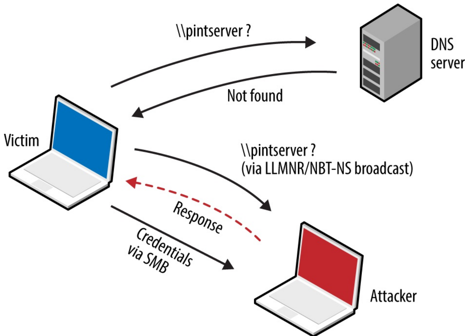
Figure 5-14. LLMNR/NBT-NS poisoning
