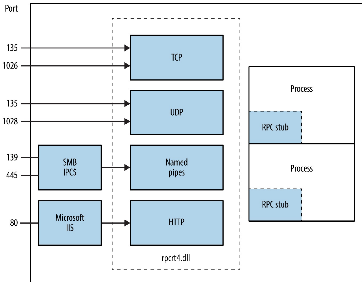
Figure 8-3. Microsoft RPC transport protocols
