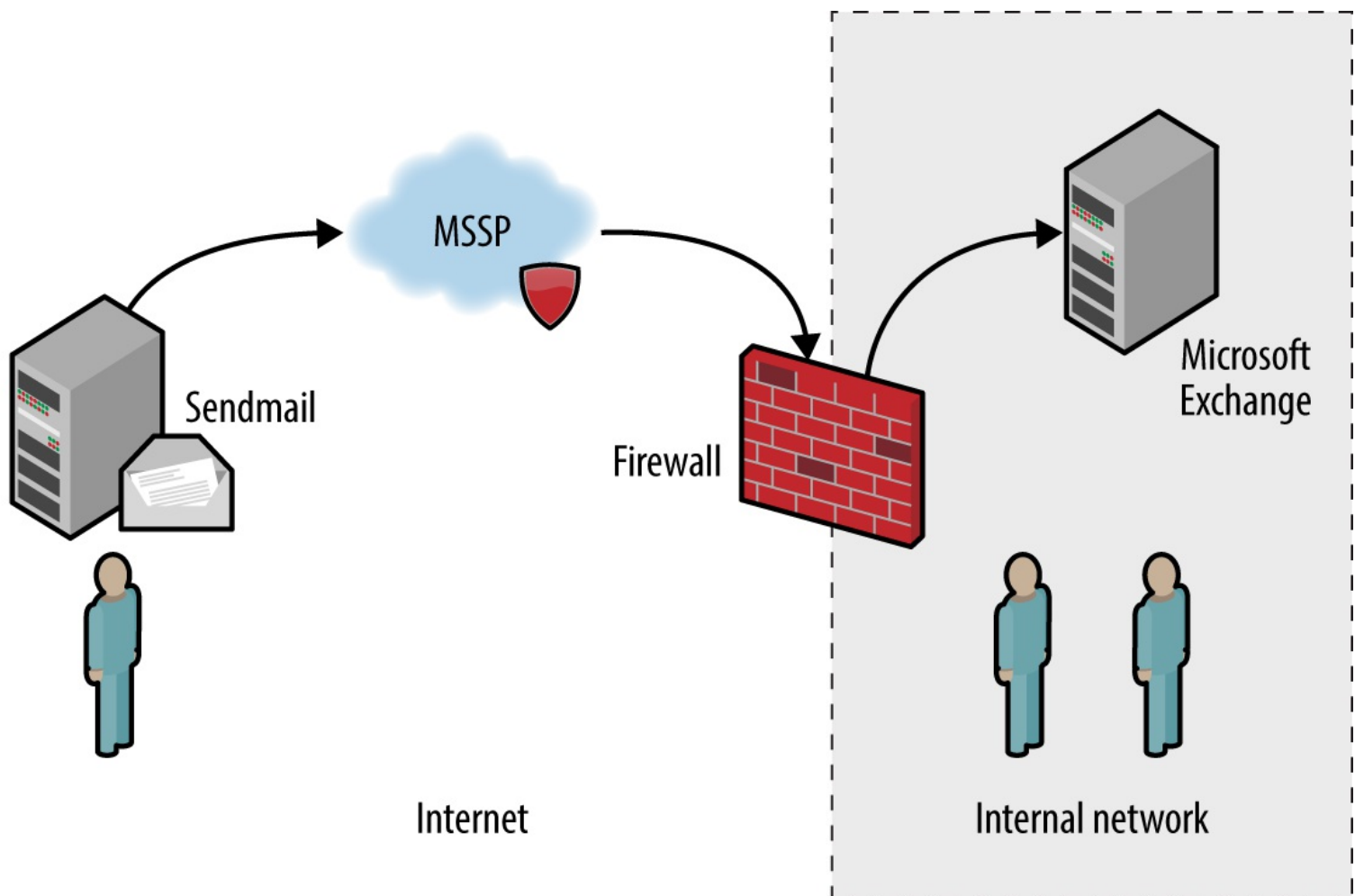
Figure 9-1. SMTP servers processing Internet-based mail
