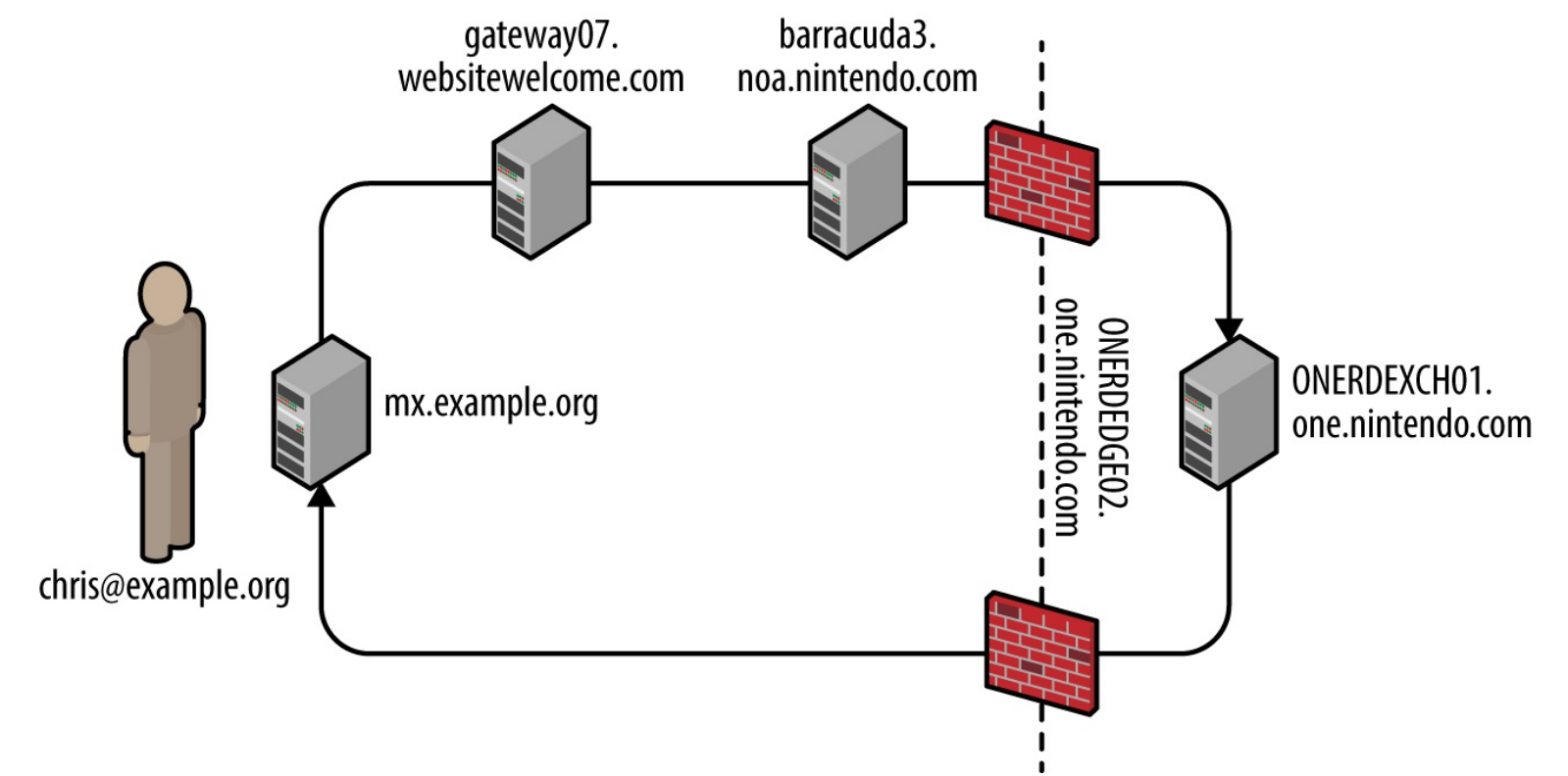
Figure 9-2. Mapping the target environment
