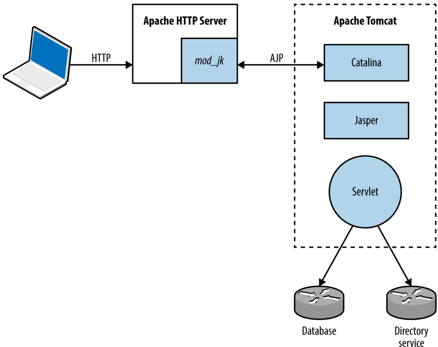
Figure 12-6. The Apache mod_jk connector in-use
