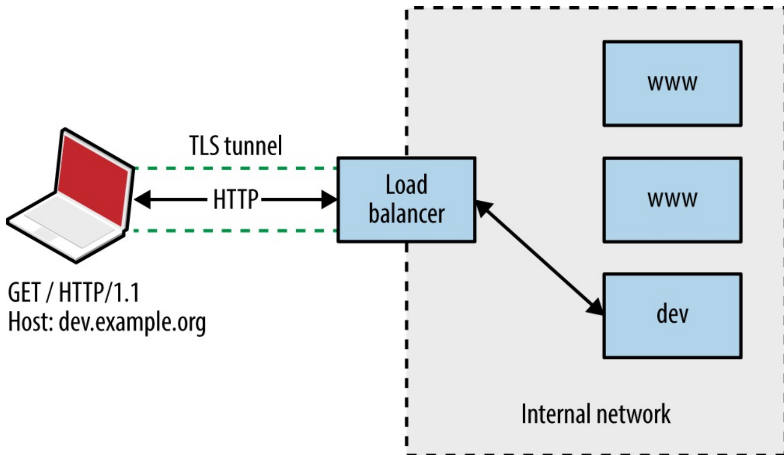
Figure 13-2. Abusing a misconfigured proxy
