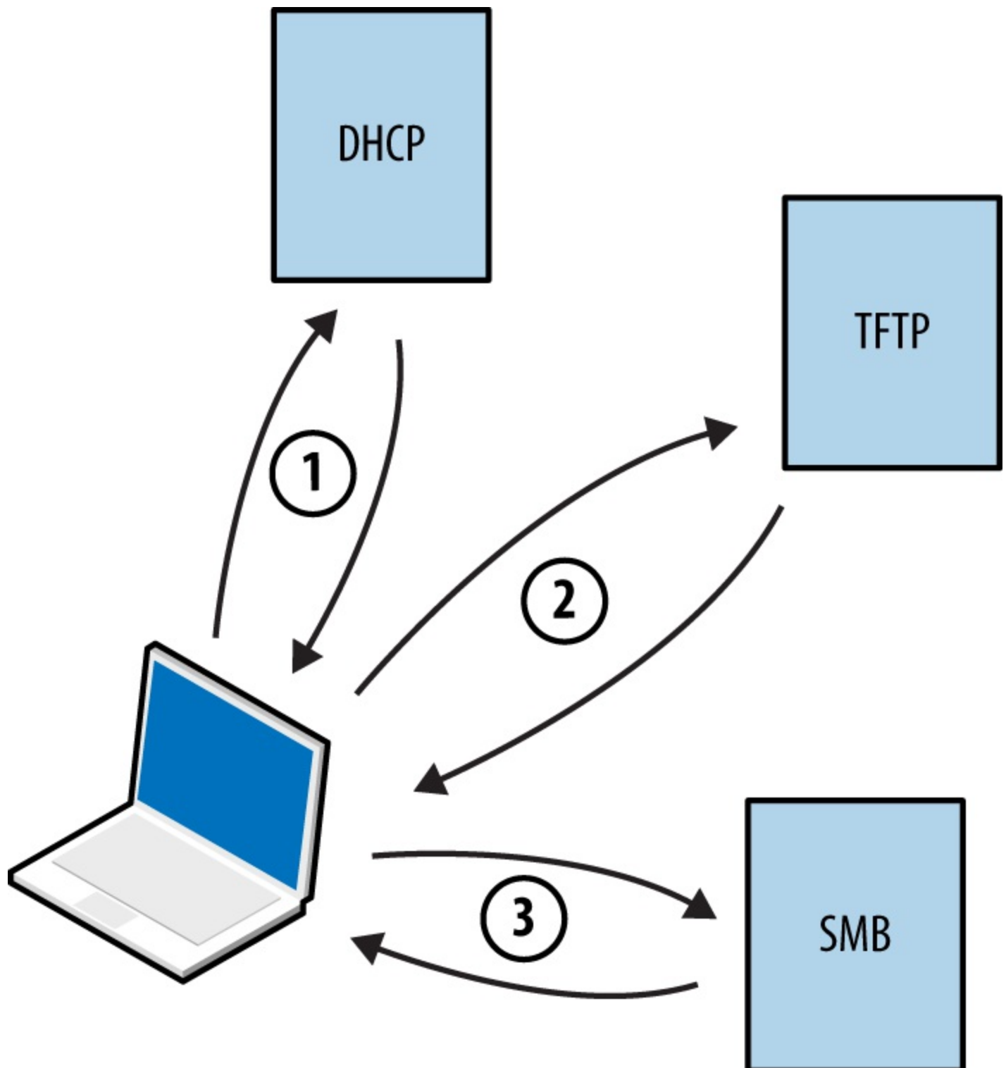
Figure 5-13. Microsoft PXE boot sequence
