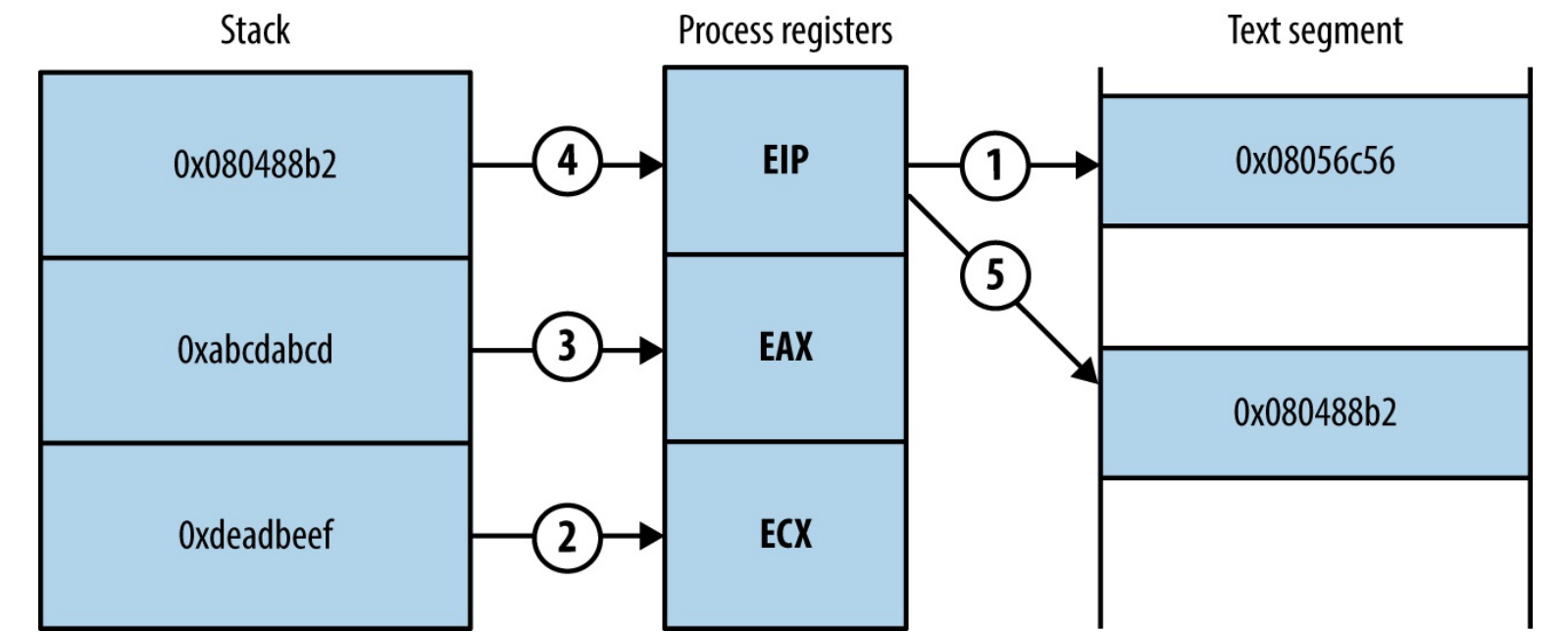
Figure 3-10. Prepared stack frame and CPU register values
