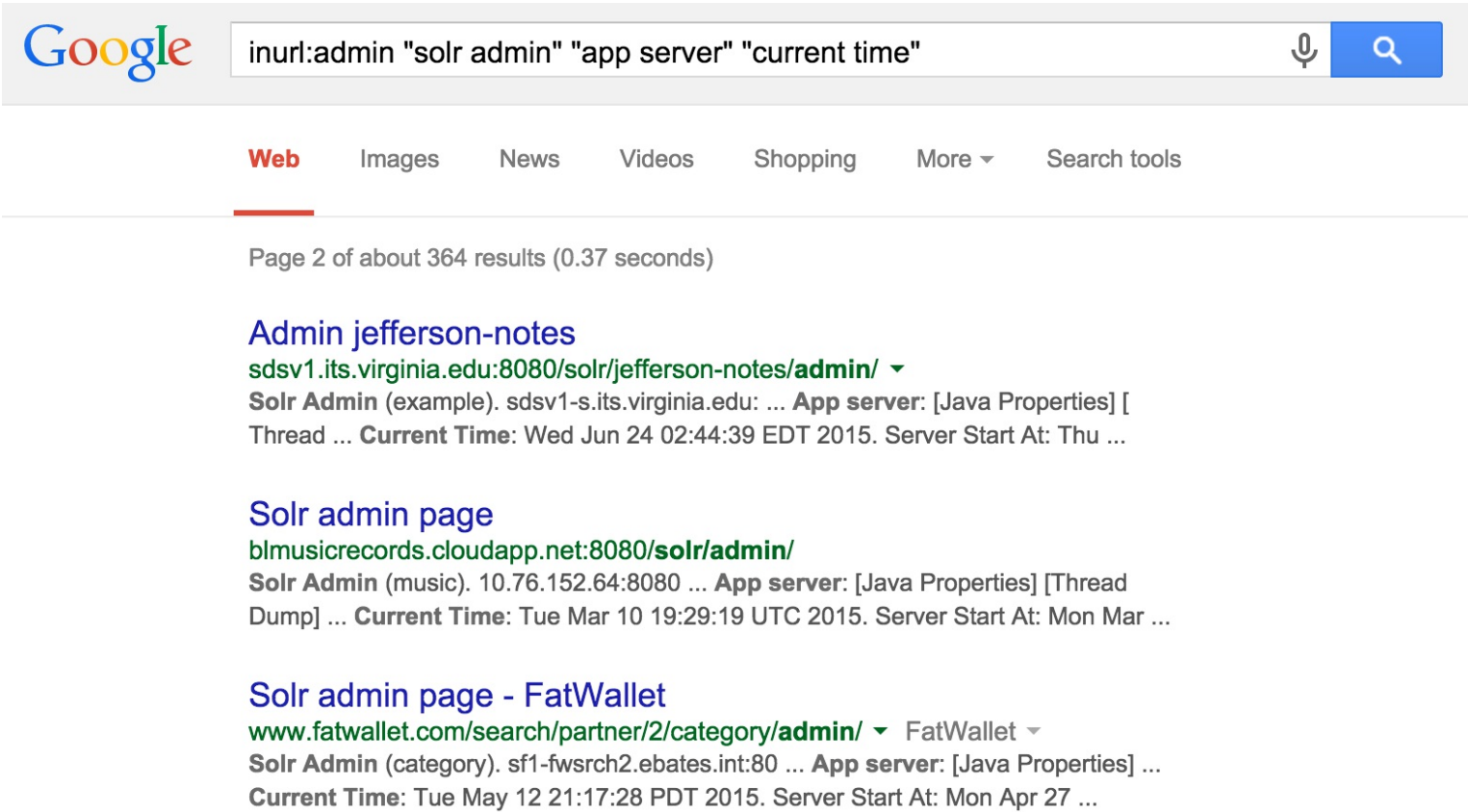
Figure 14-13. Identifying exposed Solr interfaces via Google
