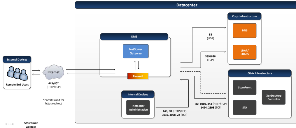
Figure 12: 1-Arm Topology
