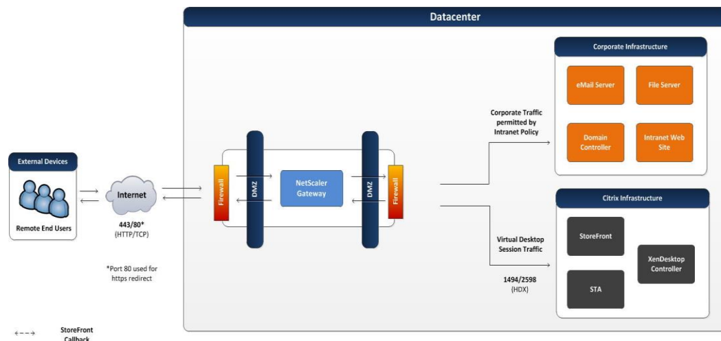
Figure 15: SSL VPN
