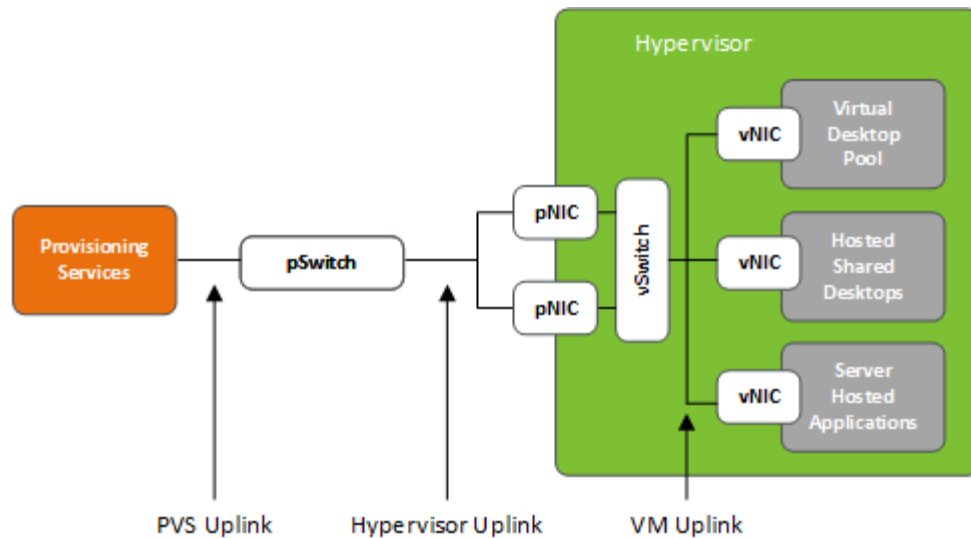
Figure 33: Sample PVS Network Configuration
