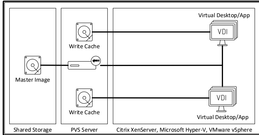
Figure 36: Server-side Local Storage Write Cache
