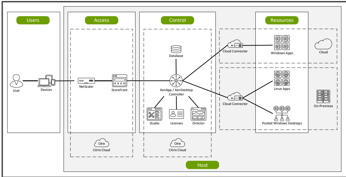
Figure 7: Citrix Cloud Architecture
