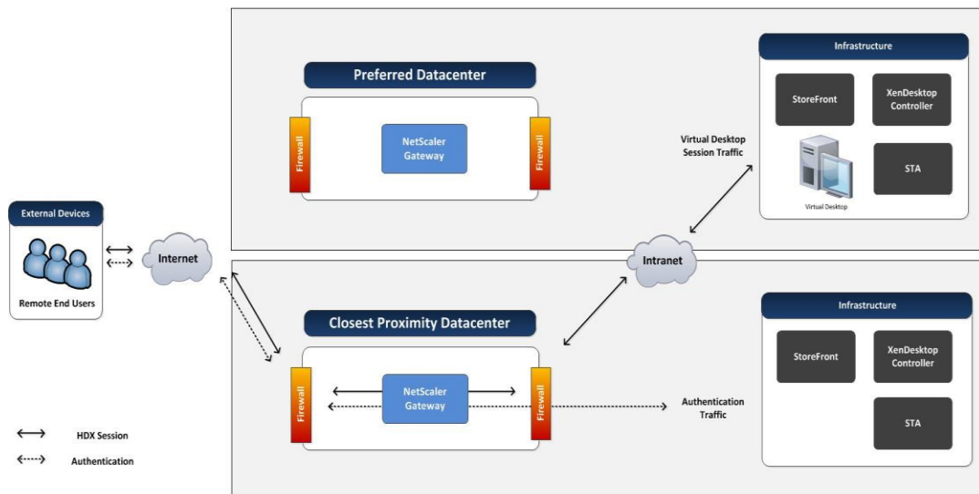
Figure 17: Intranet Connection
