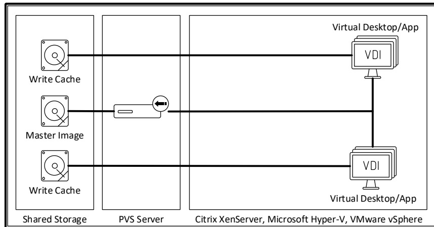
Figure 37: Server-side Shared Storage Write Cache
