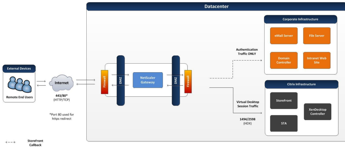
Figure 16: HDX Proxy
