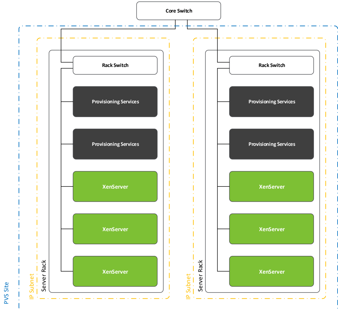
Figure 35: PVS Rack Design
