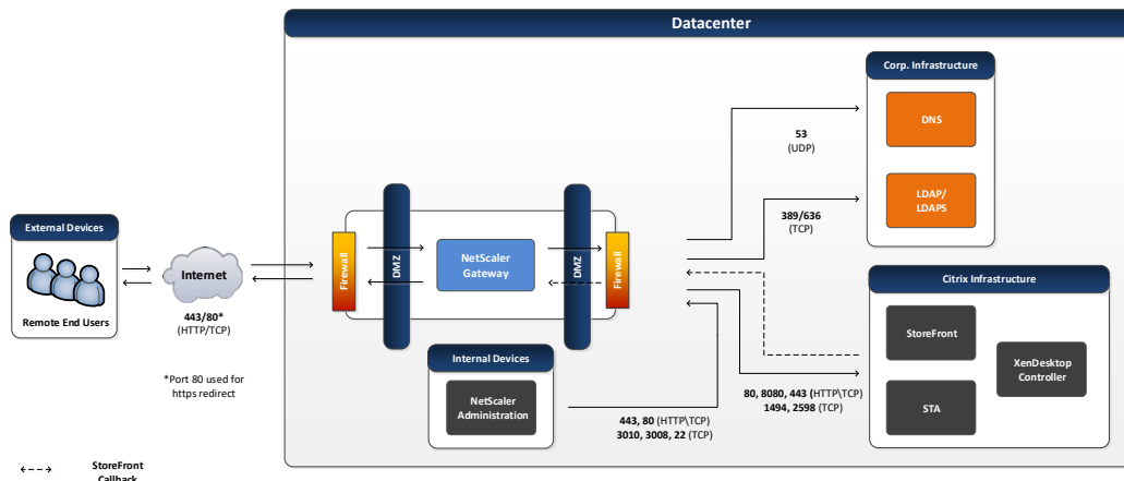
Figure 13: 2-Arm Topology
