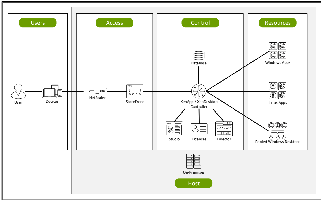
Figure 4: On-Premises Architecture
