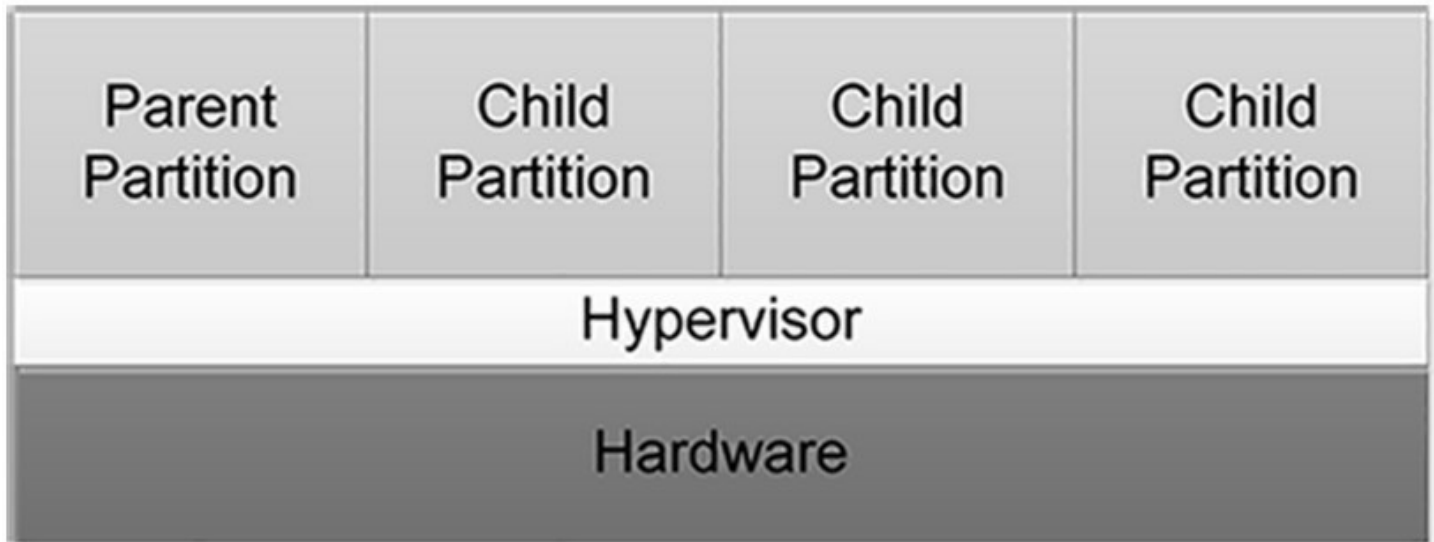
FIGURE 3-2 Type 1 virtualization
